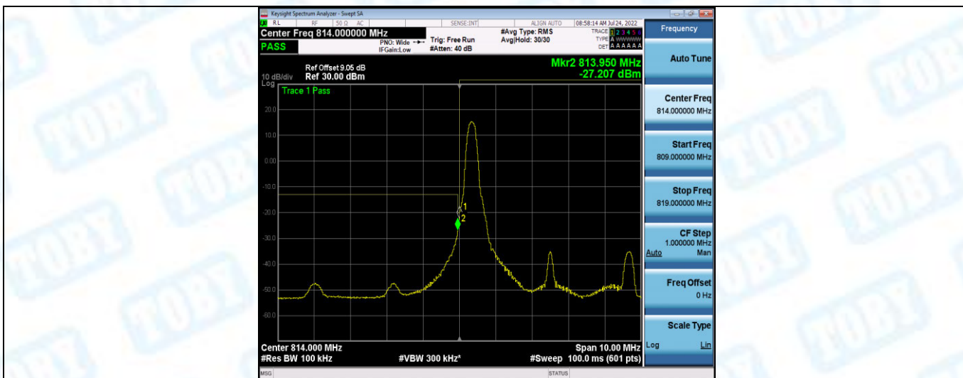
Band26-5MHz-QPSK-26715-1RB#24
