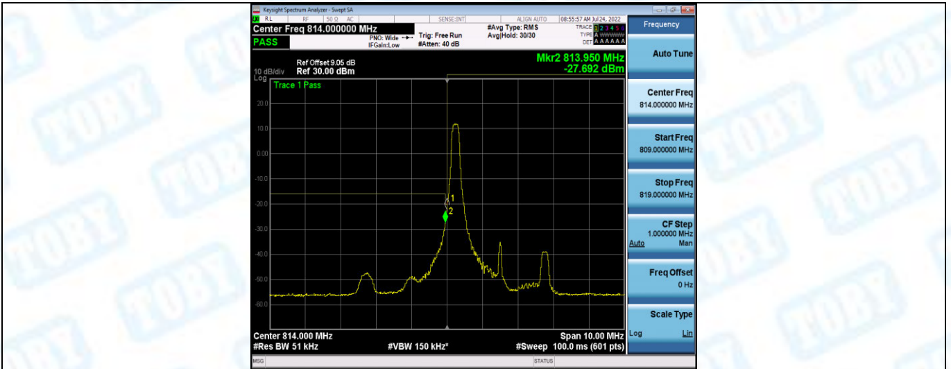
Band26-3MHz-16QAM-26705-1RB#14
