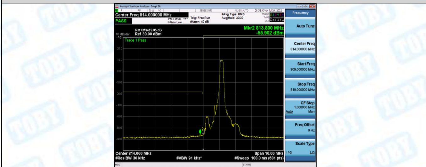
Band26-1.4MHz-16QAM-26697-6RB#0
