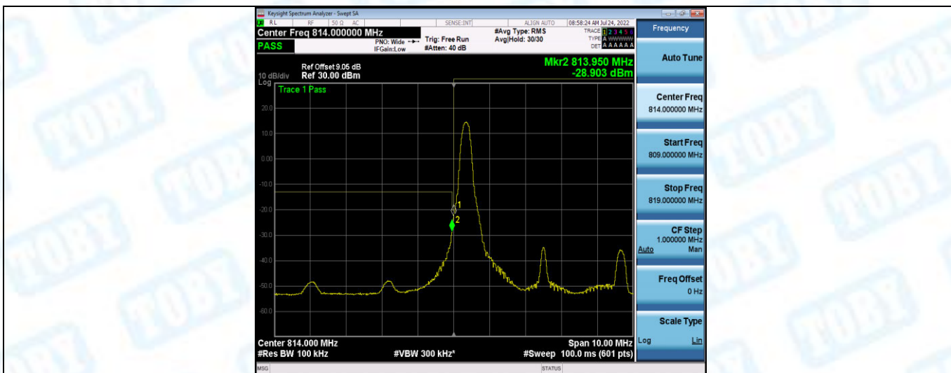
Band26-5MHz-16QAM-26715-1RB#24
