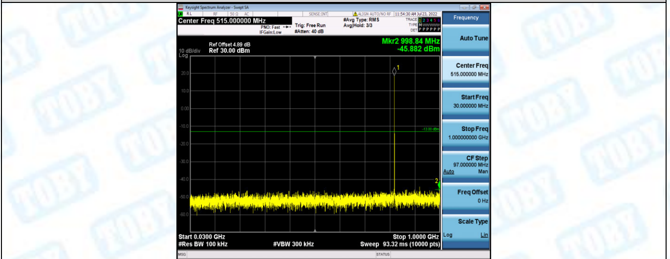
Band26-1.4MHz-16QAM-26783-1RB#0-Range2:1000~10000MHz
