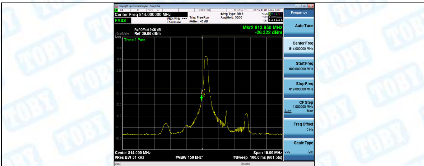
Band26-3MHz-QPSK-26705-1RB#14
