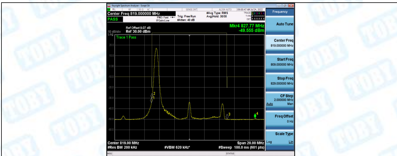
Band26-10MHz-QPSK-26740-1RB#49
