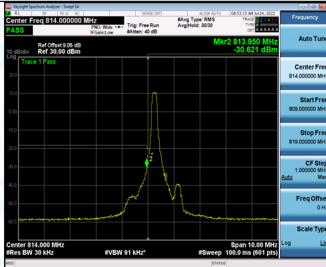
Band26-1.4MHz-QPSK-26697-1RB#5
