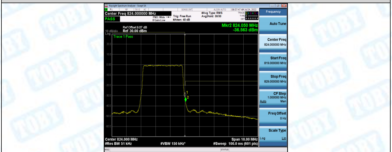
Band26-5MHz-QPSK-26715-1RB#0
