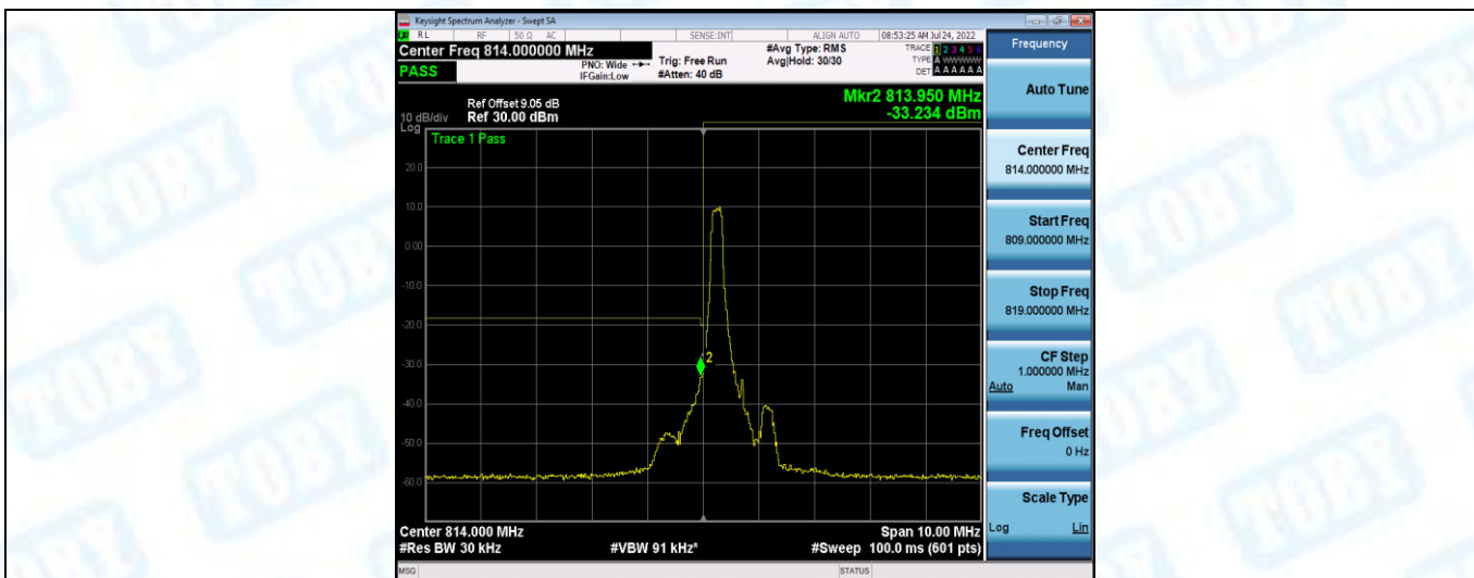
Band26-1.4MHz-16QAM-26697-1RB#5
