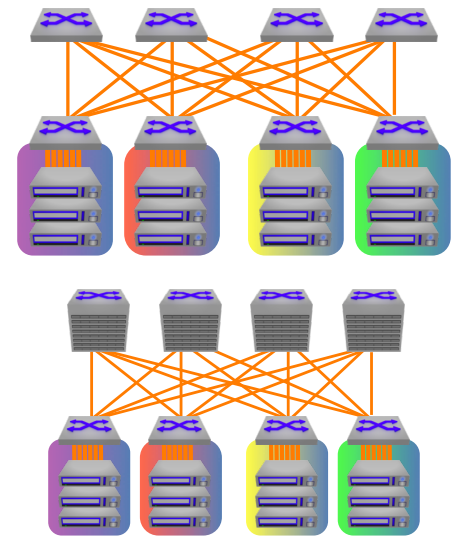
Arista Fixed System Leaf-Spine Designs Scale to 6,144 10GbE/25GbE ports or 1,536 40GbE/100GbE port at 3:1 subscription
