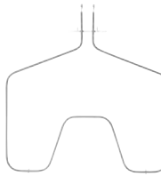
WB44X10009 (Installer Pkg) Range Oven Bake Element • 2,500/1,900 Watts • 240/208 Volts
