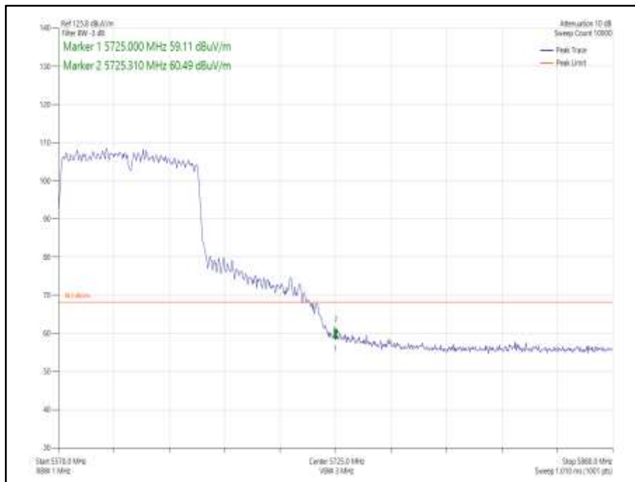
Figure 1070 - 802.11ac VHT80 CDD, Cores 0-1 - 5610 MHz Band Edge Frequency 5725 MHz
