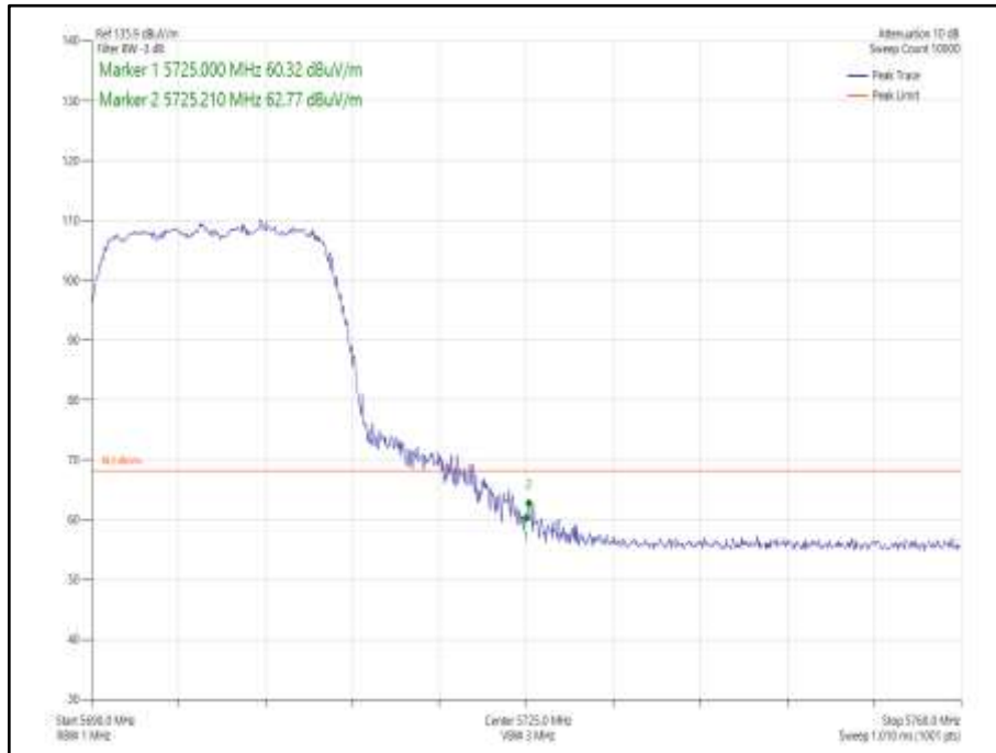
Figure 998 - 802.11n HT20 CDD, Cores 0-1 - 5700 MHz Band Edge Frequency 5725 MHz
