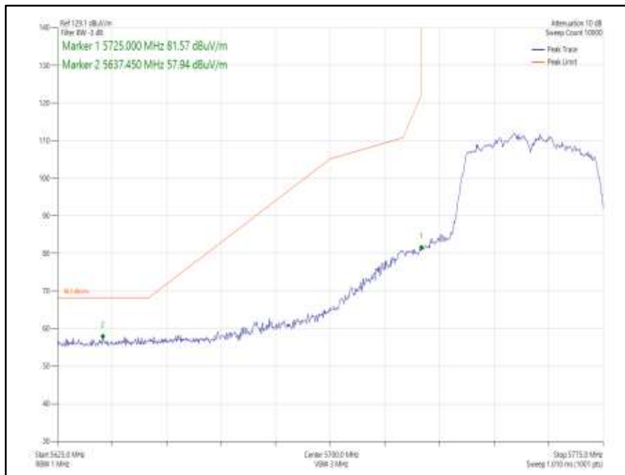
Figure 1046 - 802.11n HT40 CDD, Cores 0-1 - 5795 MHz Band Edge Frequency 5850 MHz
