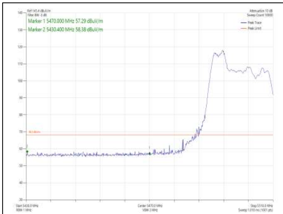
Figure 997 - 802.11ax HE20 SDM, Cores 0-1 52-37 - 5500 MHz Band Edge Frequency 5470 MHz
