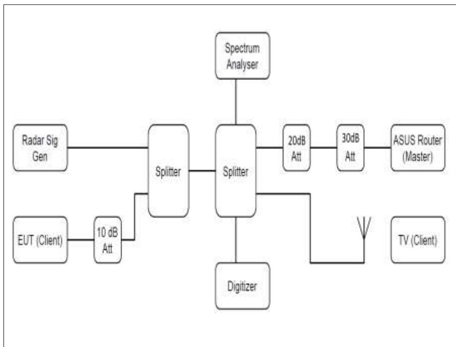
Figure 1161 - Test Equipment Setup Diagram for Client without Radar Detection with Injection at the Master
