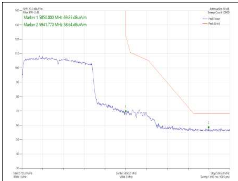
Figure 1061 - 802.11ac VHT80 Core 1 - 5775 MHz Band Edge Frequency 5850 MHz
