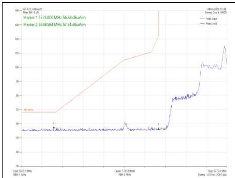
Figure 1051 - 802.11ax HE40 SDM, Cores 0-1, 26-17 - 5795 MHz Band Edge Frequency 5850 MHz
