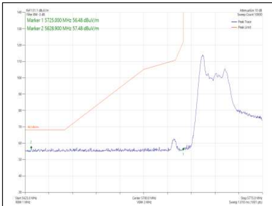
Figure 1043 - 802.11ax HE40 CDD, Cores 0-1, 26-0 - 5755 MHz Band Edge Frequency 5725 MHz
