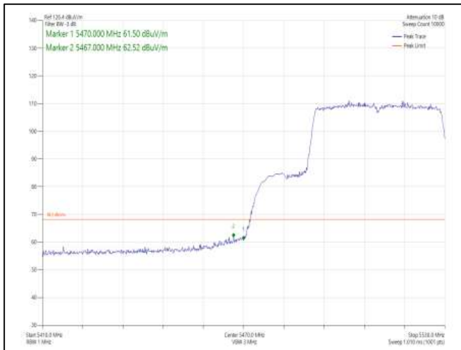
Figure 1017 - 802.11ax HE40, Core 1, SU - 5510 MHz Band Edge Frequency 5470 MHz
