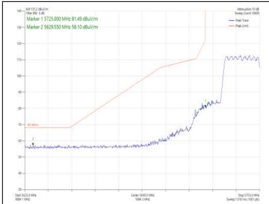
Figure 1006 - - 802.11ax HE20 CDD, Cores 0-1, SU - 5745 MHz Band Edge Frequency 5725 MHz
