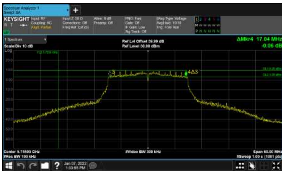
Figure 951 - Core 1 (B) 5745 MHz (CH149) 6 dB Bandwidth
