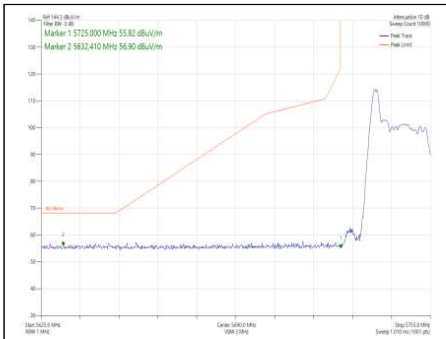
Figure 987- 802.11ax HE20, Core 1, 26-0 - 5745 MHz Band Edge Frequency 5735 MHz
