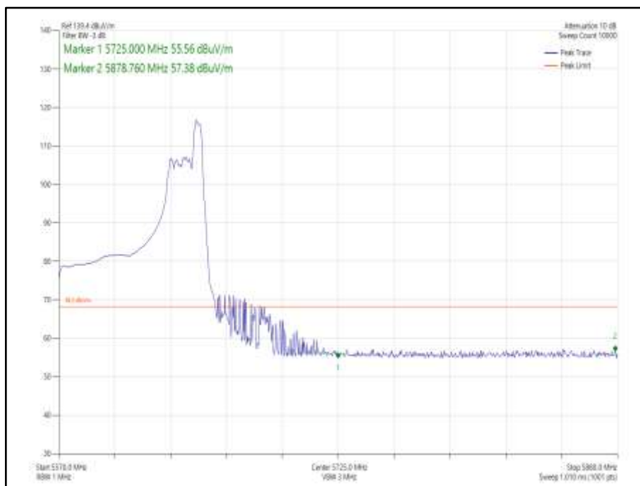
Figure 1075 - 802.11ax HE80 SDM, Cores 0-1, 26-36 - 5610 MHz Band Edge Frequency 5725 MHz
