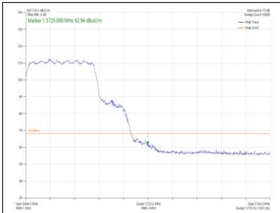
Figure 1000 - - 802.11ax HE20 CDD, Cores 0-1, SU - 5700 MHz Band Edge Frequency 5725 MHz
