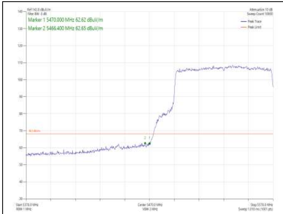
Figure 1068 - 802.11ax HE80 SDM, Cores 0-1, SU - 5530 MHz Band Edge Frequency 5470 MHz
