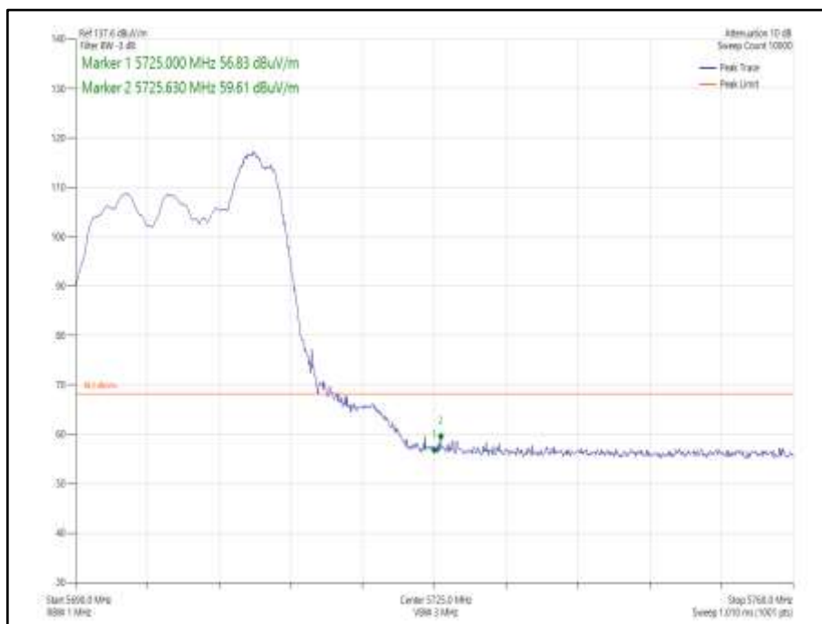
Figure 1001 - 802.11ax HE20 CDD, Cores 0-1, 52-40 - 5700 MHz Band Edge Frequency 5725 MHz
