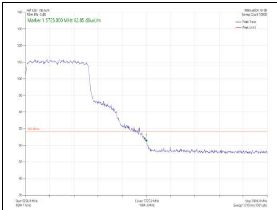
Figure 1036 - 802.11ax HE40 CDD, Cores 0-1, SU - 5670 MHz Band Edge Frequency 5725 MHz
