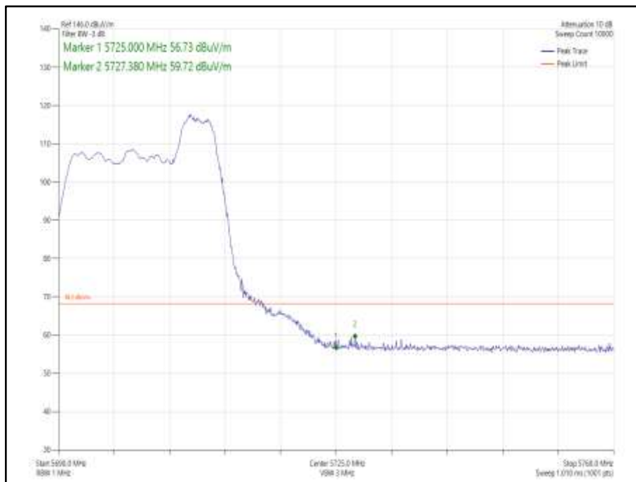
Figure 1003 - 802.11ax HE20 SDM, Cores 0-1, 52-40 - 5700 MHz Band Edge Frequency 5725 MHz
