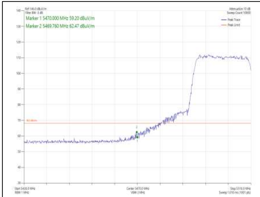
Figure 996 - - 802.11ax HE20 SDM, Cores 0-1 SU - 5500 MHz Band Edge Frequency 5470 MHz
