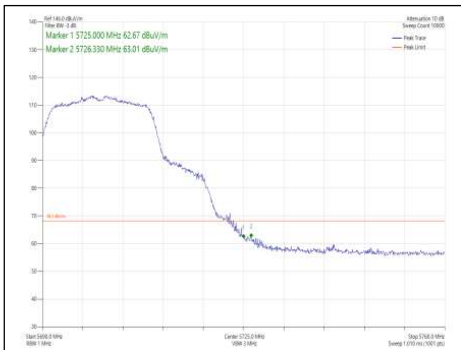
Figure 981 - 802.11n HT20, Core 1 - 5700 MHz Band Edge Frequency 5725 MHz
