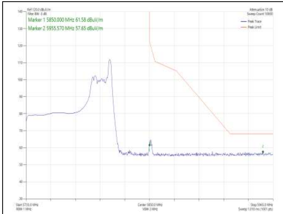
Figure 1063 - 802.11ax HE80 Core 1 26-36 - 5775 MHz Band Edge Frequency 5850 MHz
