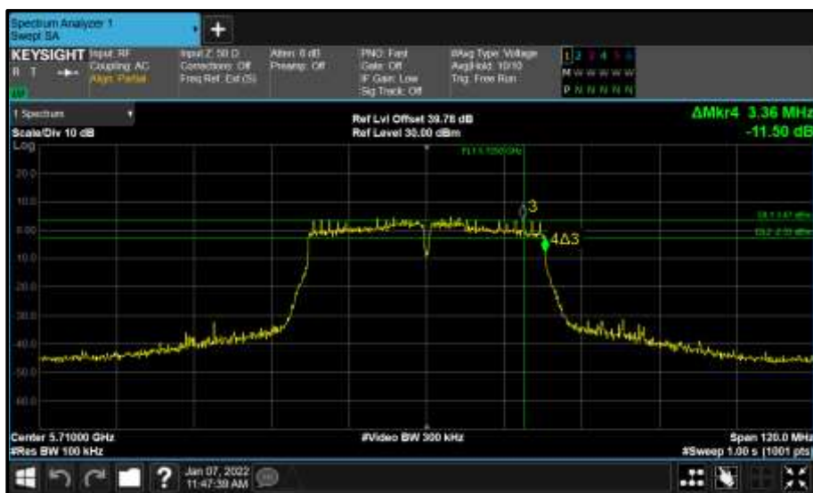
Figure 961 - Core 0 (A) 5710 MHz (CH142) 6 dB Bandwidth
