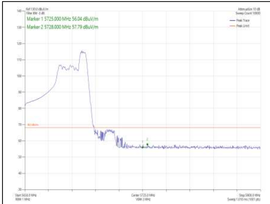
Figure 1021 - 802.11ax HE40, Core 1, 52-44 - 5670 MHz Band Edge Frequency 5725 MHz
