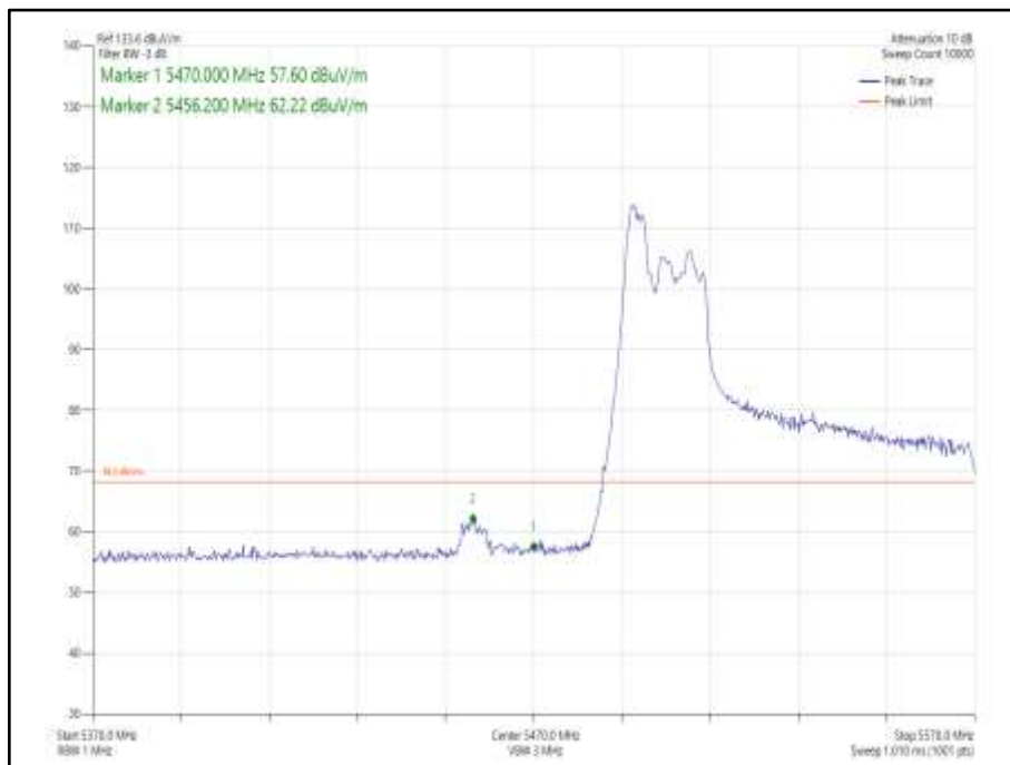
Figure 1069 - 802.11ax HE80 SDM, Cores 0-1, 52-37 - 5530 MHz Band Edge Frequency 5470 MHz
