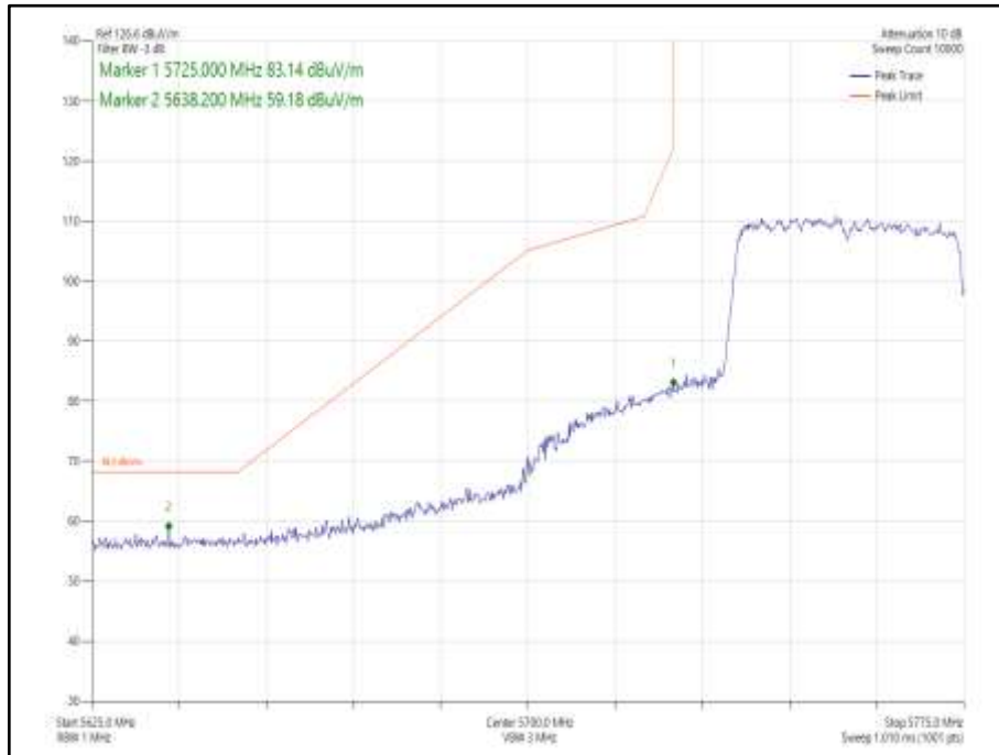
Figure 1042 - 802.11ax HE40 CDD, Cores 0-1, SU - 5755 MHz Band Edge Frequency 5725 MHz
