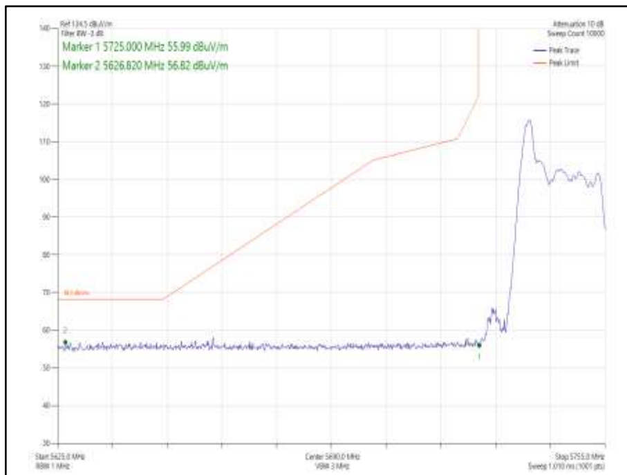
Figure 1007 - 802.11ax HE20 CDD, Cores 0-1, 26-0 - 5745 MHz Band Edge Frequency 5725 MHz
