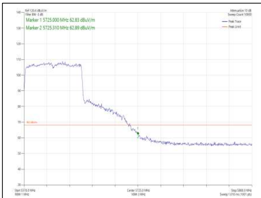
Figure 1071 - 802.11ac VHT80 SDM, Cores 0-1 - 5610 MHz Band Edge Frequency 5725 MHz
