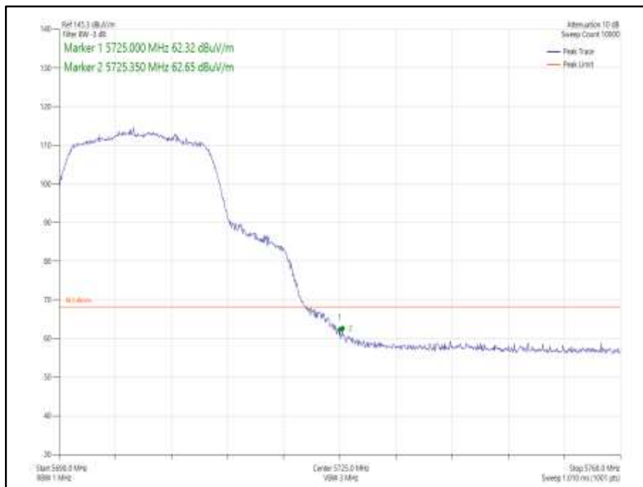
Figure 999 - 802.11n HT20 SDM, Cores 0-1 - 5700 MHz Band Edge Frequency 5725 MHz
