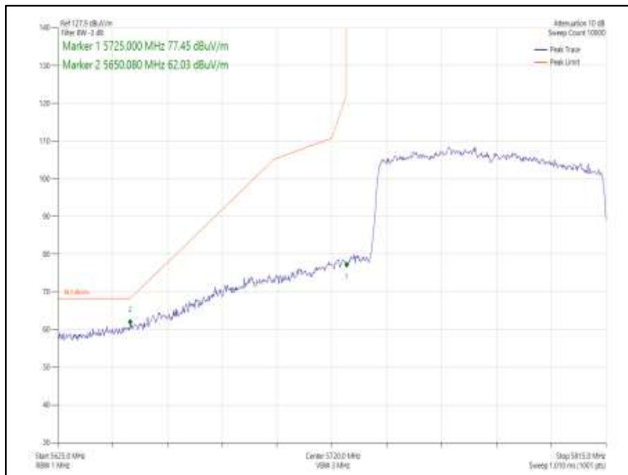
Figure 1080 - 802.11ax HE80 SDM, Cores 0-1, SU - 5775 MHz Band Edge Frequency 5725 MHz
