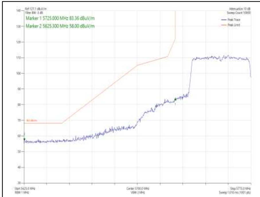
Figure 1050 - 802.11ax HE40 SDM, Cores 0-1, SU - 5795 MHz Band Edge Frequency 5850 MHz
