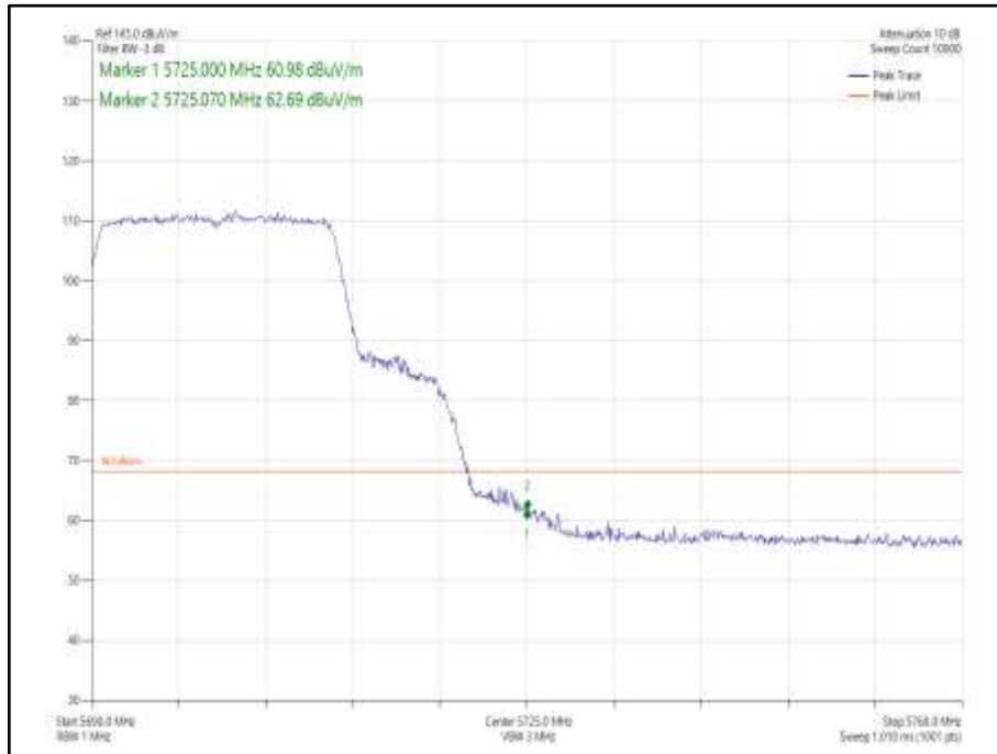
Figure 1002 - - 802.11ax HE20 SDM, Cores 0-1, SU - 5700 MHz Band Edge Frequency 5725 MHz
