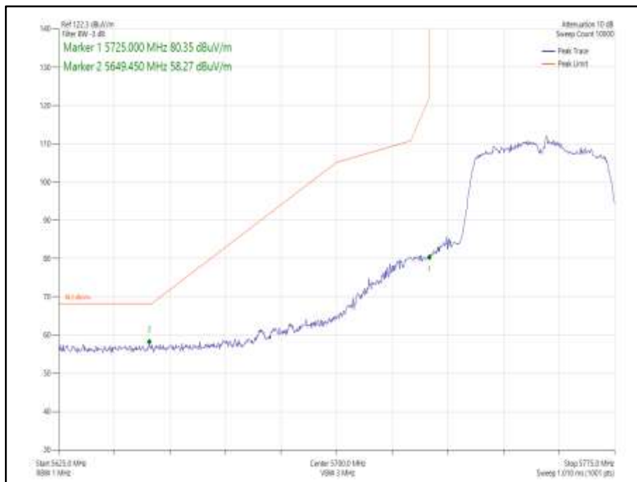
Figure 1022 - 802.11n HT40, Core 1 - 5755 MHz Band Edge Frequency 5725 MHz
