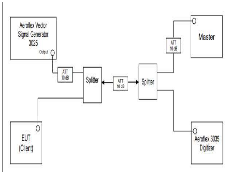
Figure 1155 - Test Equipment Setup Diagram for Client without Radar Detection with Injection at the Master
