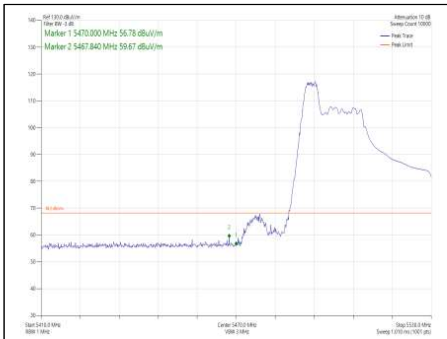
Figure 1018 - 802.11ax HE40, Core 1, 52-37 - 5510 MHz Band Edge Frequency 5470 MHz
