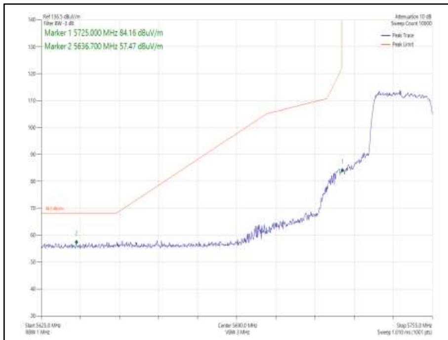
Figure 986- 802.11ax HE20, Core 1, SU - 5745 MHz Band Edge Frequency 5735 MHz
