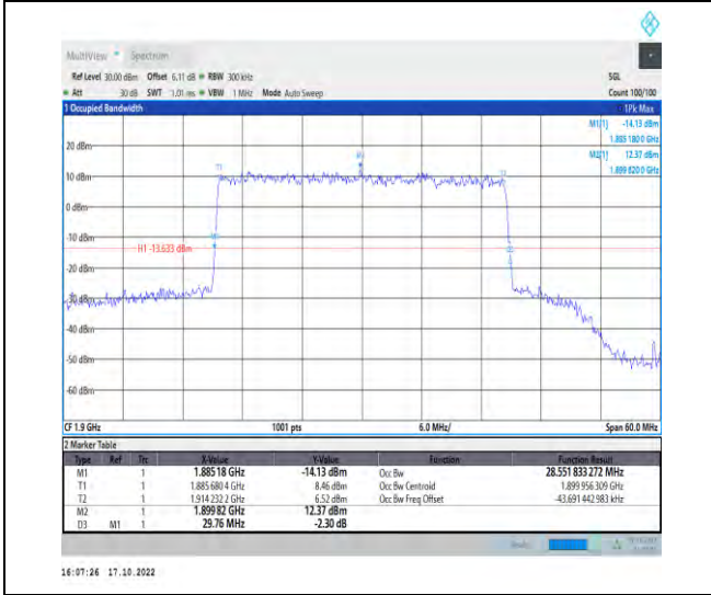
1-N25-PC3-15-30-H-4-DFT-64QAM-Outer_Full-160 @0-Ant1-28.552-29.760-≤30-PASS
