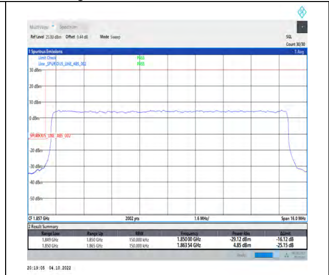
1-N25-PC3-15-15-L-3-DFT-QPSK-Outer_Full-75@0-Ant1-1-seegraph-PASS-see graph
