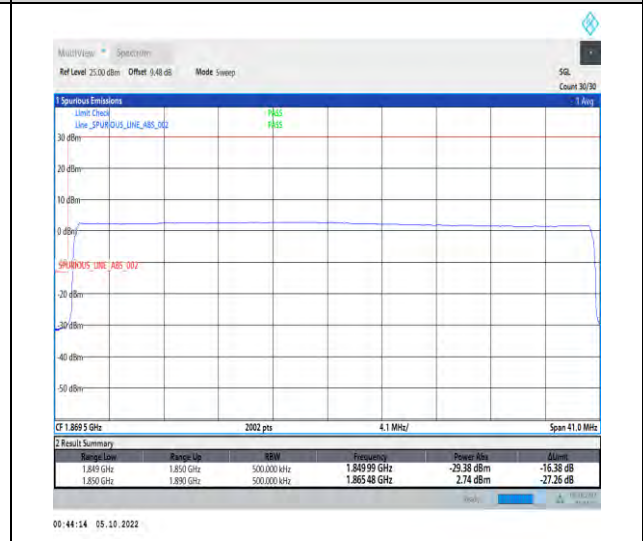
1-N25-PC3-15-40-L-6-CP-QPSK-Outer_Full-216@ 0-Ant1-1-seegraph-PASS-see graph
