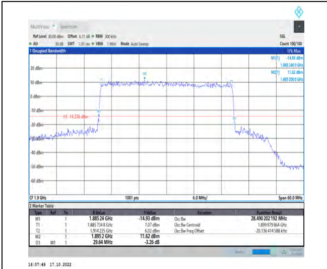
1-N25-PC3-15-30-H-6-CP-QPSK-Outer_Full-160@0 -Ant1-28.49-29.640-≤30-PASS
