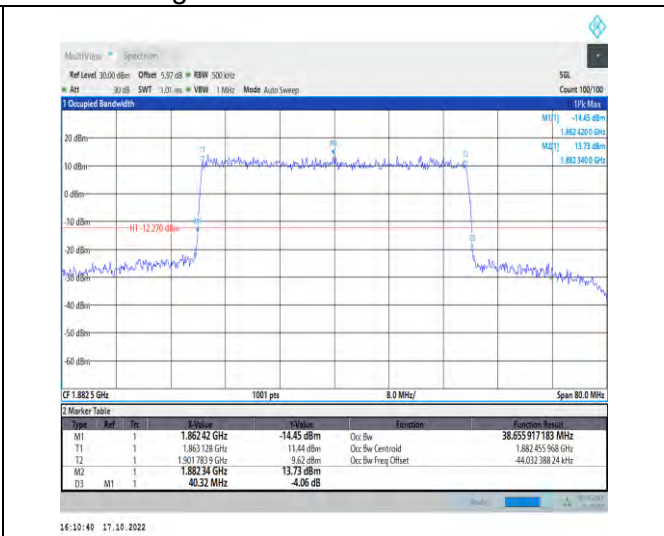
1-N25-PC3-15-40-M-3-DFT-16QAM-Outer_Full-216 @0-Ant1-38.656-40.320-≤40-PASS
