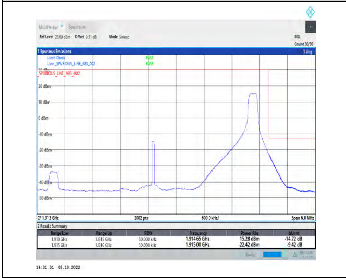
1-N25-PC3-15-5-H-5-CP-QPSK-Edge_1RB_Right-1@24-Ant1-1-seegraph-PASS-see graph
