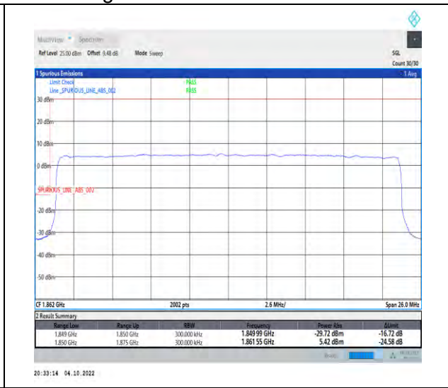
1-N25-PC3-15-25-L-3-DFT-QPSK-Outer_Full-128@0-Ant1-1-seegraph-PASS-see graph
