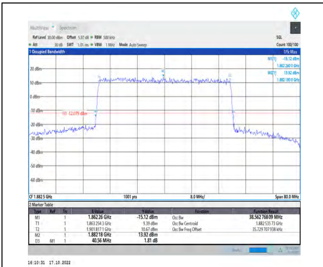
1-N25-PC3-15-40-M-1-DFT-QPSK-Outer_Full-216@ 0-Ant1-38.563-40.560-≤40-PASS
