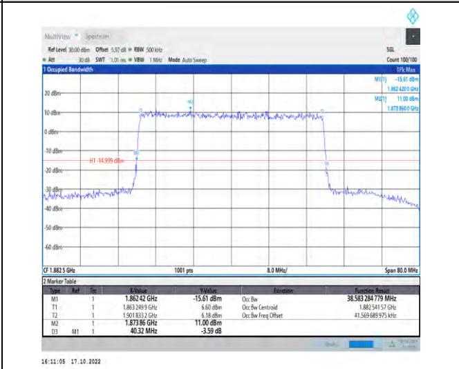
1-N25-PC3-15-40-M-5-DFT-256QAM-Outer_Full-216 @0-Ant1-38.583-40.320-≤40-PASS
