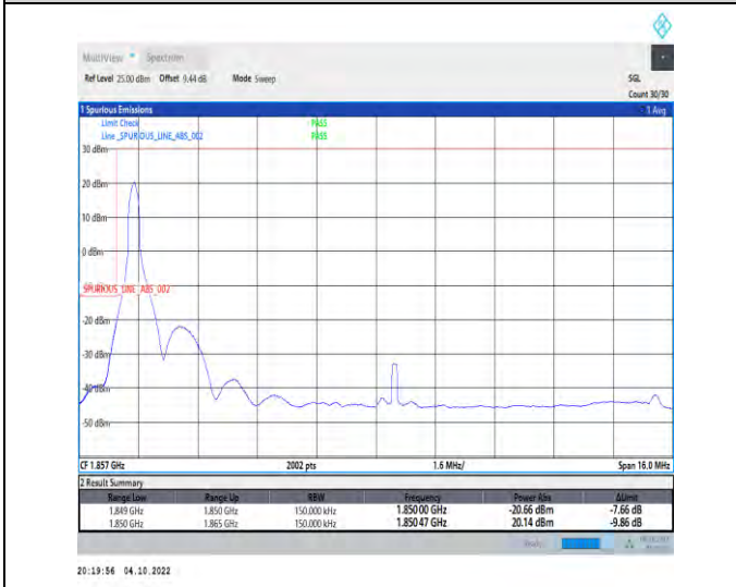
1-N25-PC3-15-15-L-4-CP-QPSK-Edge_1RB_Left-1@0-Ant1-1-seegraph-PASS-see graph
