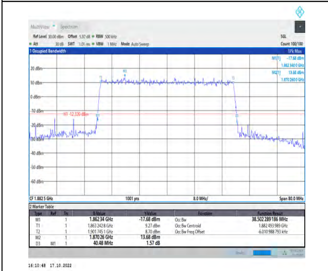
1-N25-PC3-15-40-M-4-DFT-64QAM-Outer_Full-216 @0-Ant1-38.502-40.480-≤40-PASS
