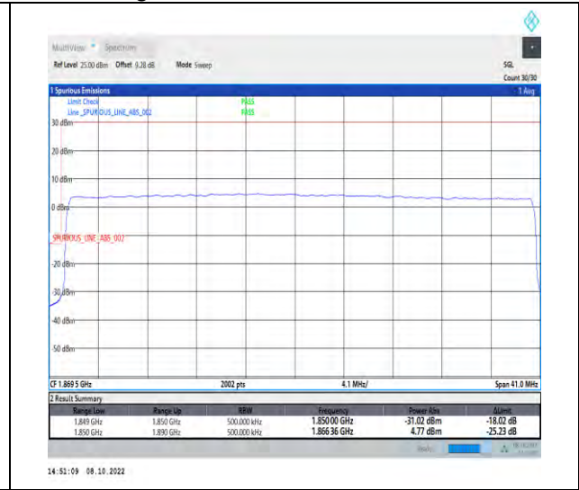
1-N25-PC3-15-40-L-3-DFT-QPSK-Outer_Full-216@ 0-Ant1-1-seegraph-PASS-see graph
