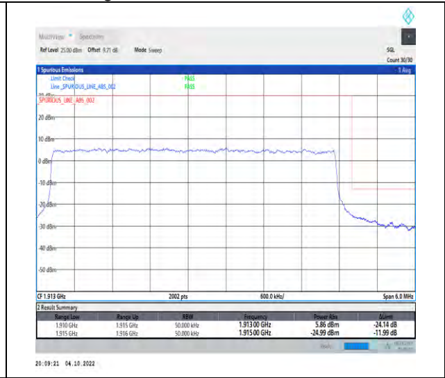
1-N25-PC3-15-5-H-3-DFT-QPSK-Outer_Full-25@0-Ant1-1-seegraph-PASS-see graph
