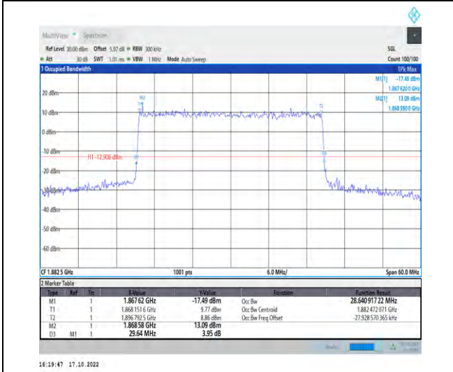
1-N25-PC3-15-30-M-4-DFT-64QAM-Outer_Full-160 @0-Ant1-28.641-29.640-≤30-PASS
