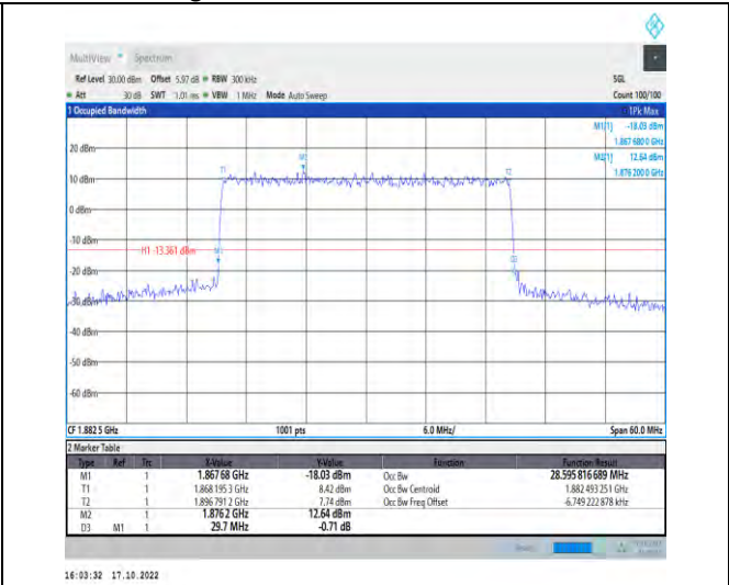
1-N25-PC3-15-30-M-3-DFT-16QAM-Outer_Full-160 @0-Ant1-28.596-29.700-≤30-PASS
