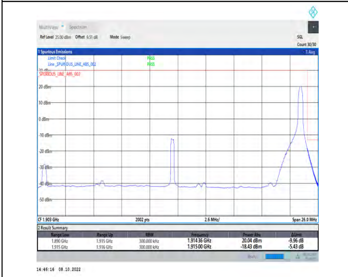
1-N25-PC3-15-25-H-5-CP-QPSK-Edge_1RB_Right-1 @132-Ant1-1-seegraph-PASS-see graph
