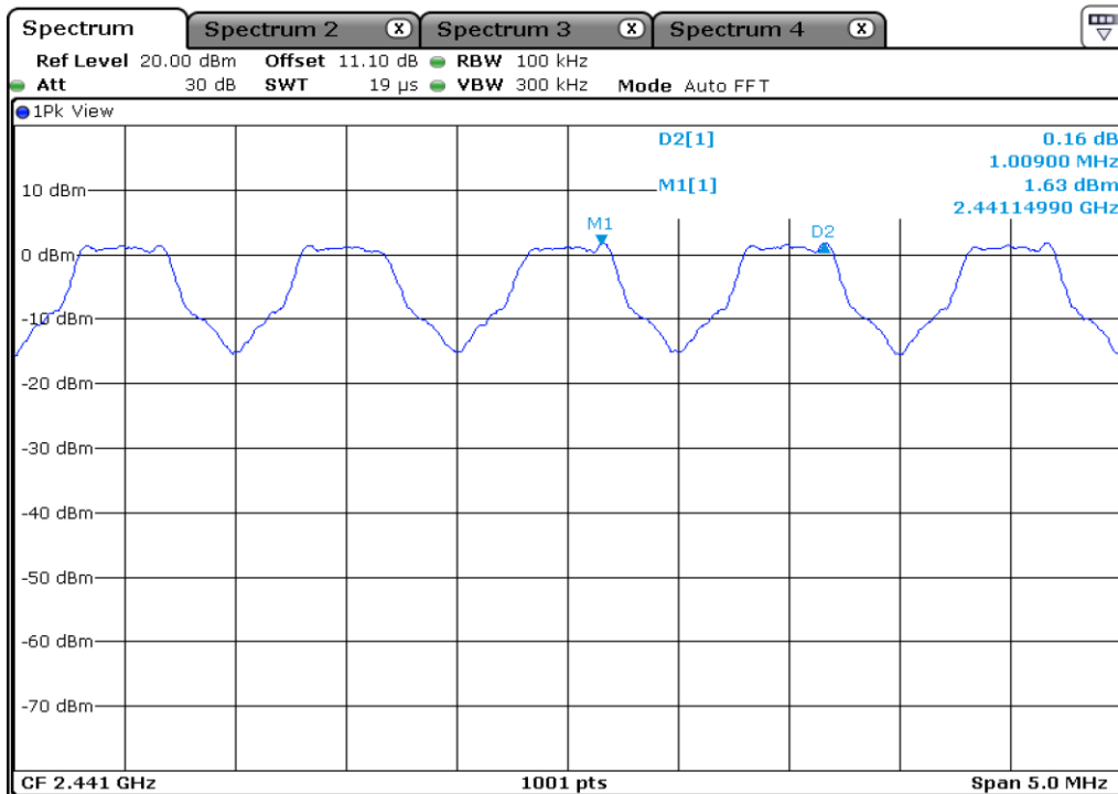
1 | Hopping Frequency Separation
