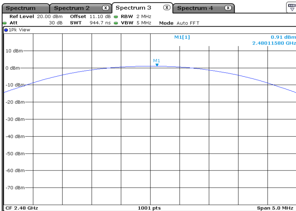
6 Maimum Peak Output Power
