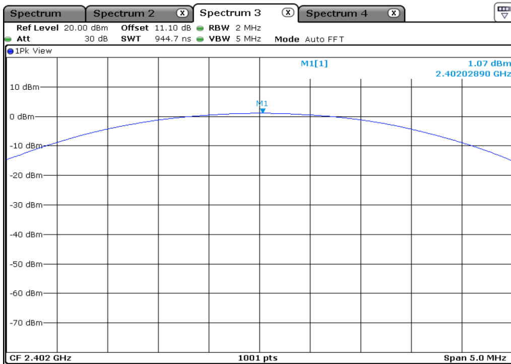
7 Maimum Peak Output Power
