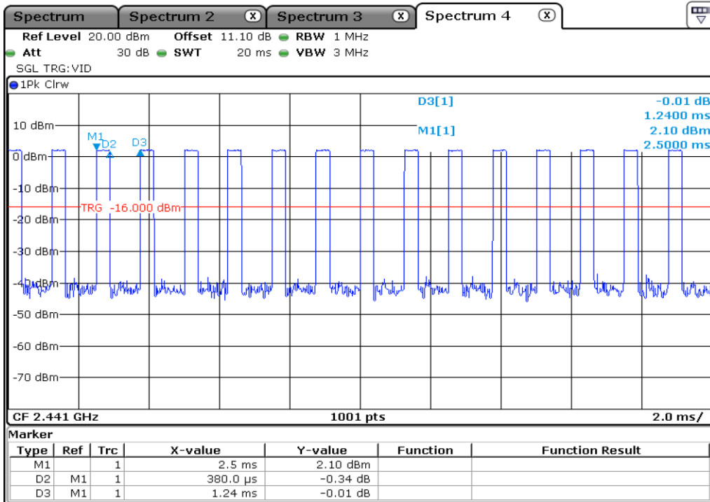
1 Time Of Occupancy
