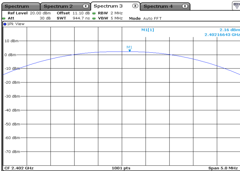
1 Maimum Peak Output Power
