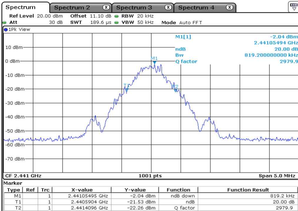
2 Minimum 20 dB Bandwidth
