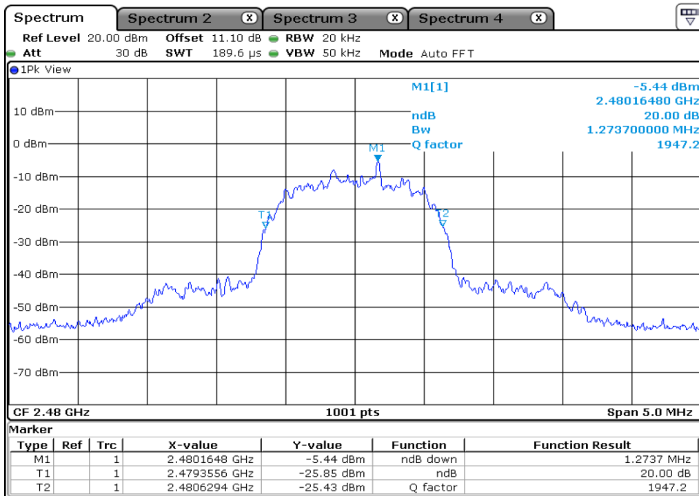
9 Minimum 20 dB Bandwidth
