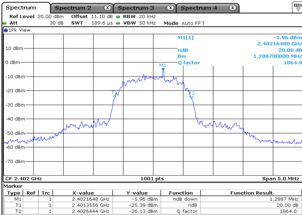
7 Minimum 20 dB Bandwidth
