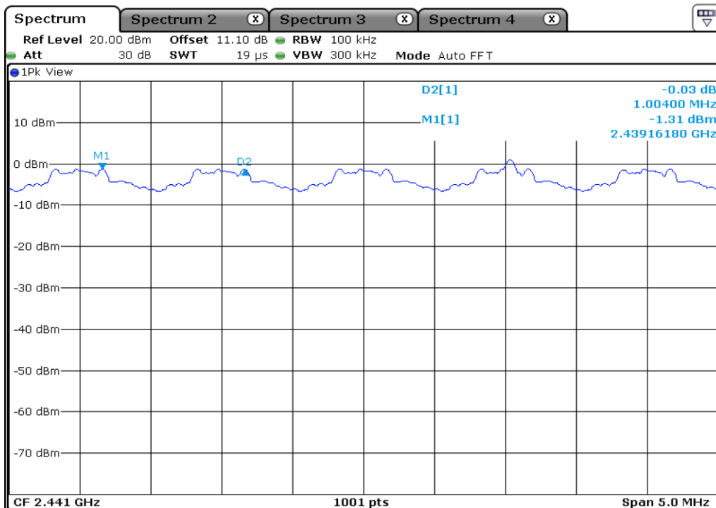
2 | Hopping Frequency Separation
