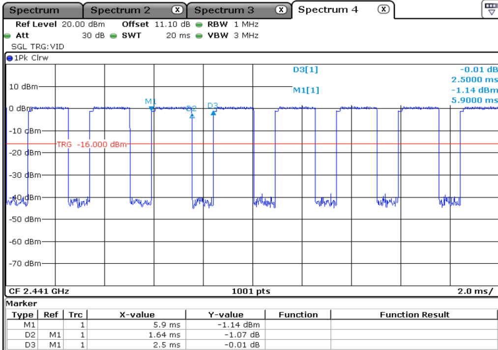
8 Time Of Occupancy
