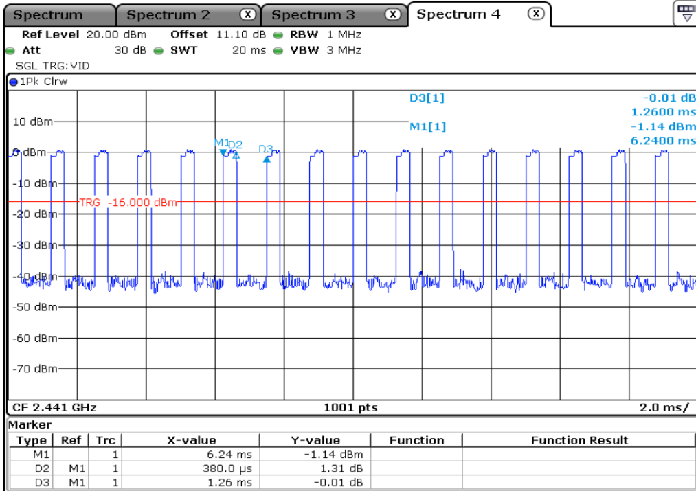
7 Time Of Occupancy
