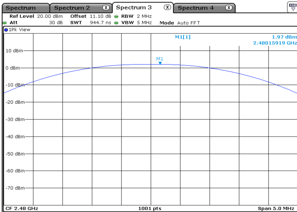
3 Maimum Peak Output Power
