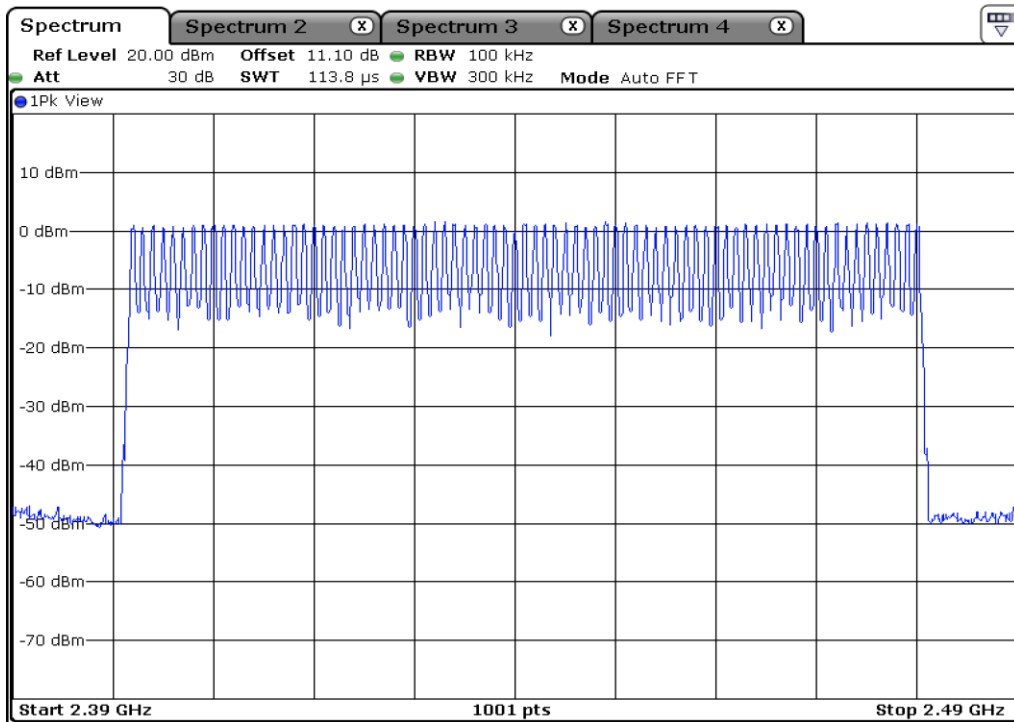
1 Number Of Hopping Channels
