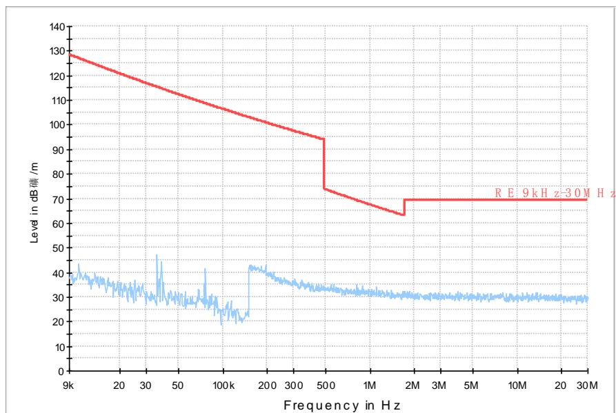
RE 9kHz-30MHz
