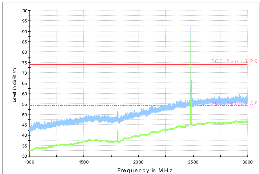
RE - 1GHz-3GHz
