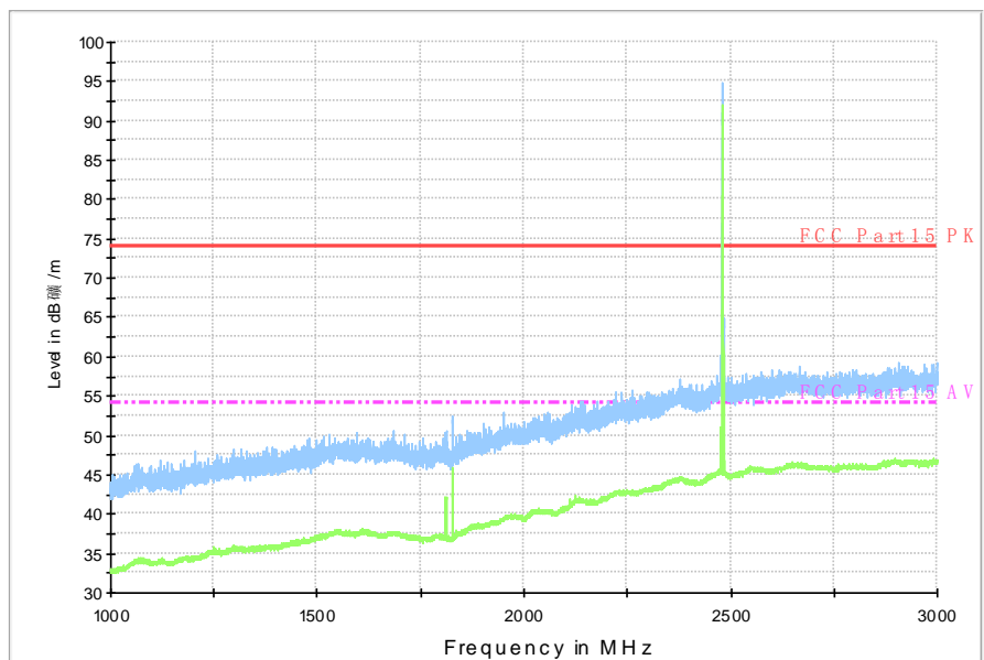
RE - 1GHz-3GHz
