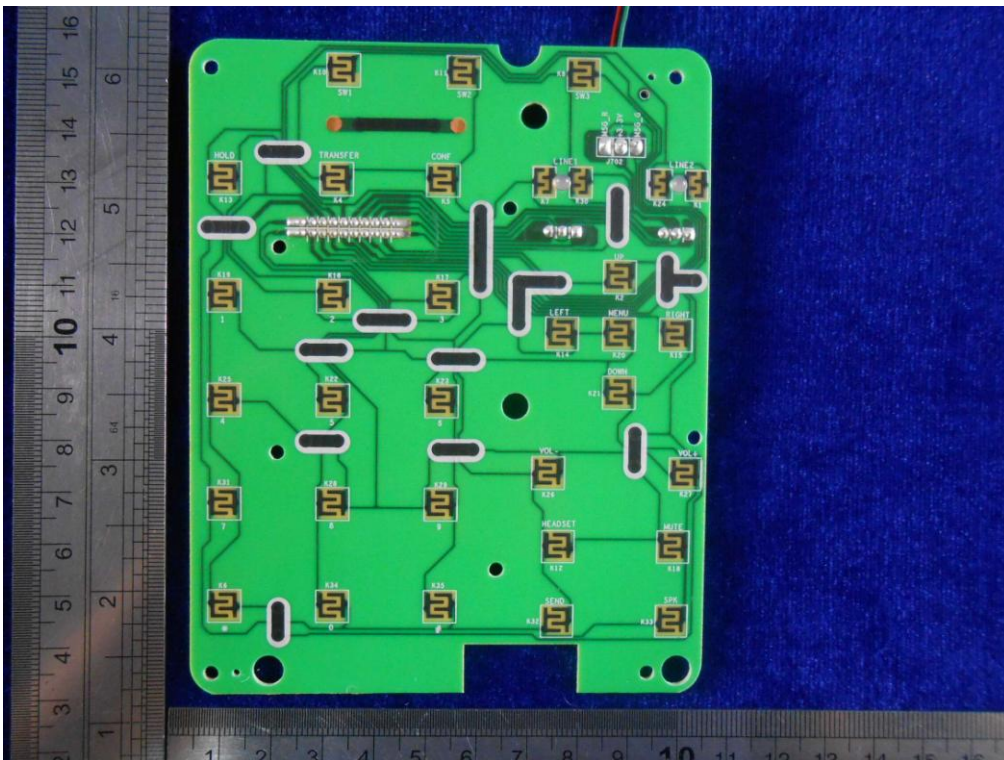
EUT-Uncovered View 4
