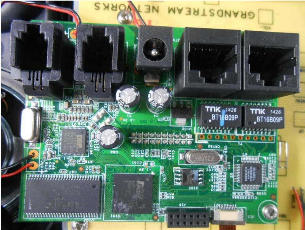
Mainboard-Top View
