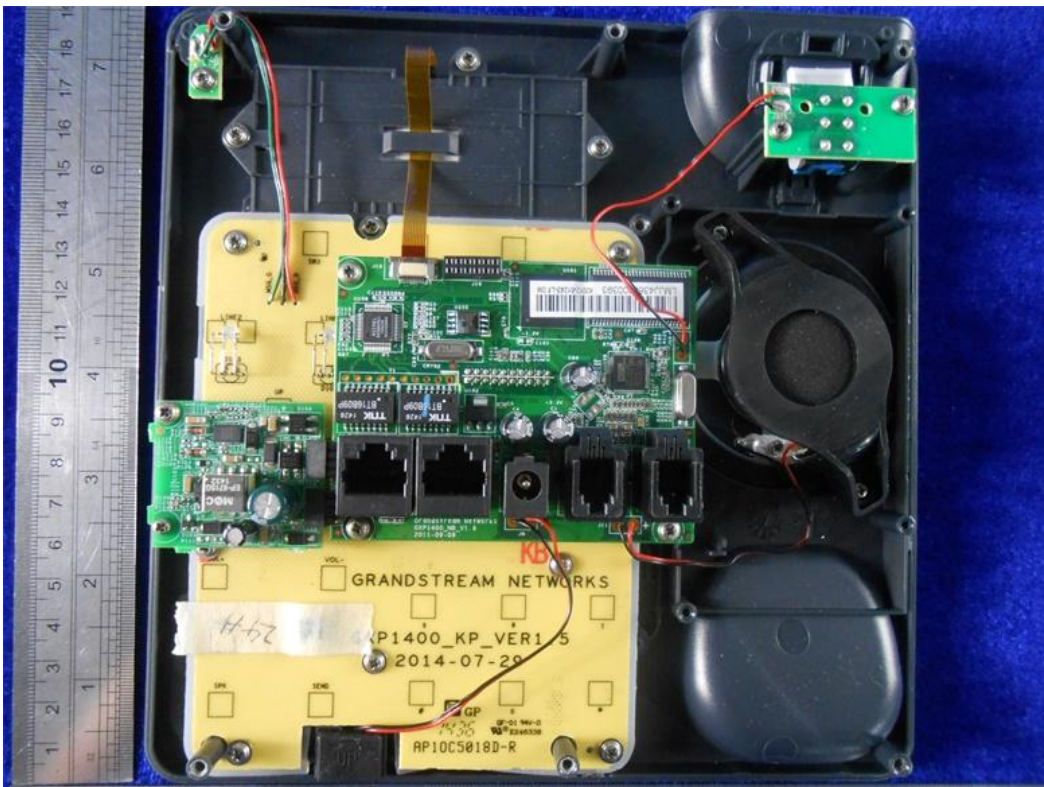
EUT-Uncovered View 02
