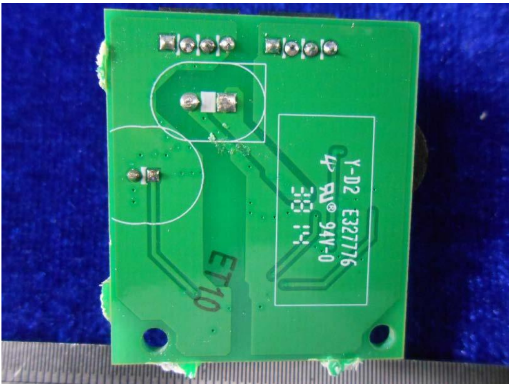
PoE Board-Bottom View
