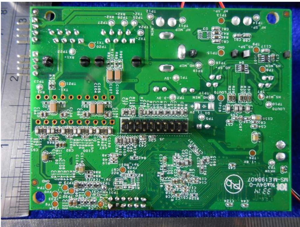
Mainboard-Bottom View
