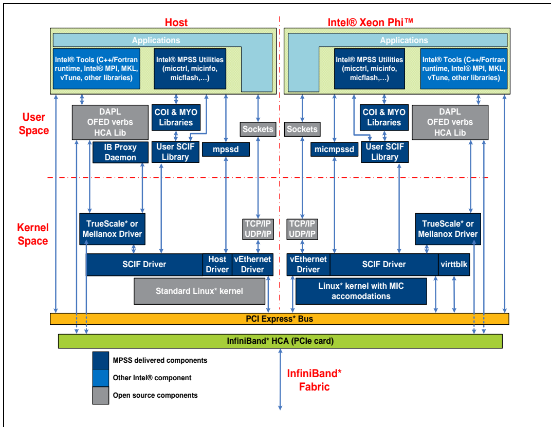
Figure 5: Intel® MPSS Architecture
