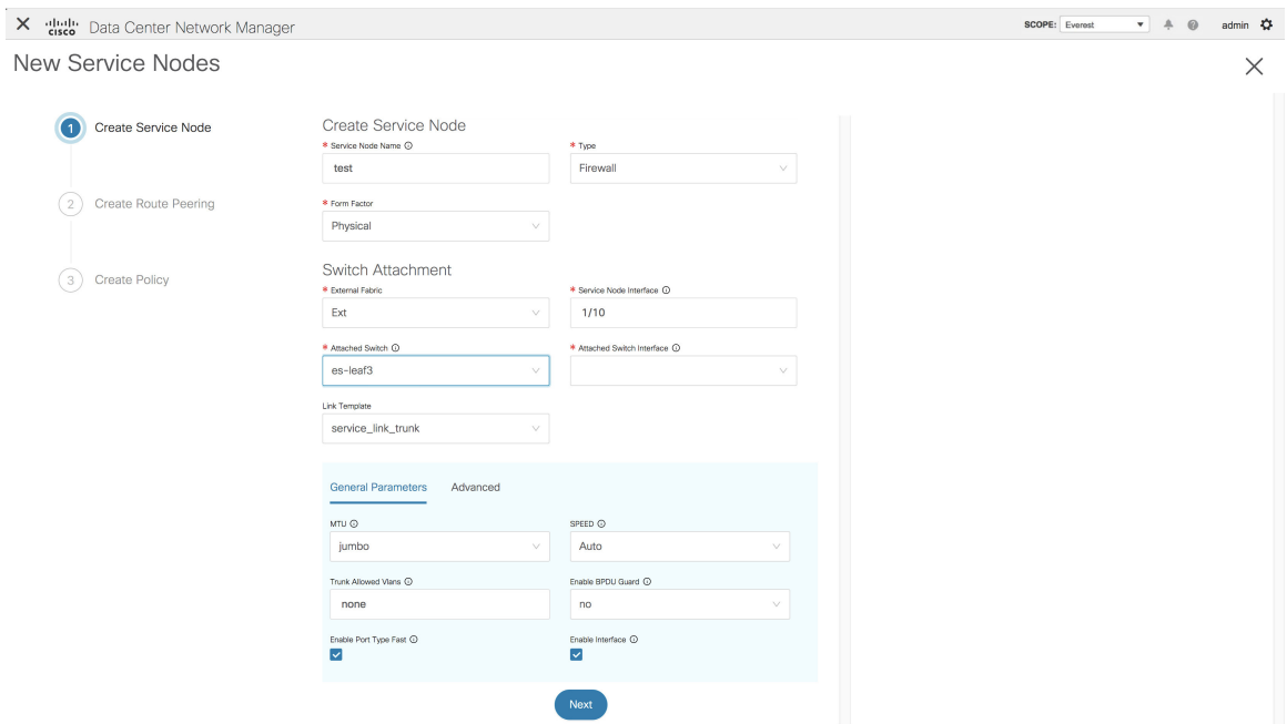
Figure 10: Example: Link Template - service_link_trunk
