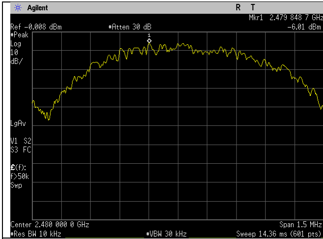
High Ch_2480MHz_1MBit_Spectral Density
