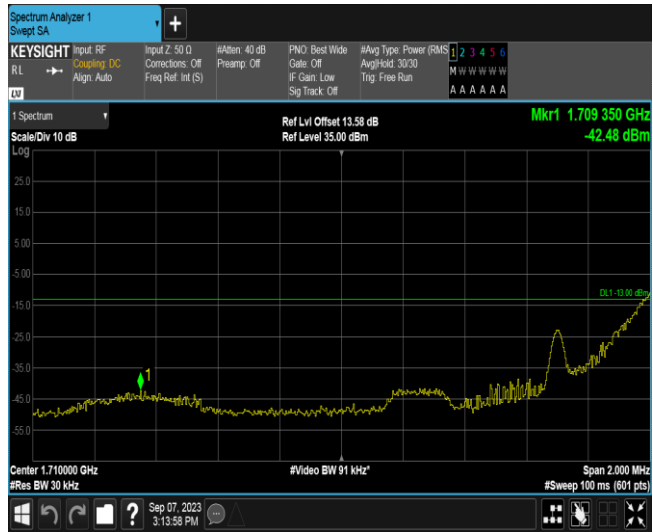
Band4-1.4MHz-16QAM-19957-6RB#0
