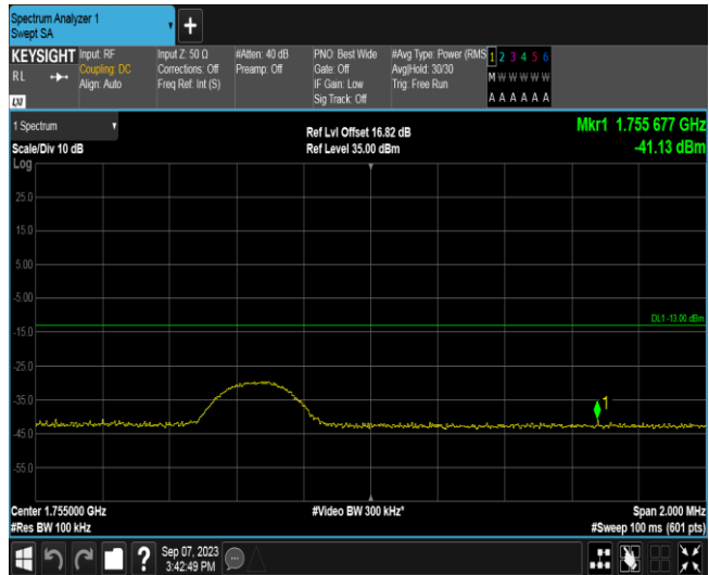
Band4-5MHz-16QAM-20375-1RB#24
