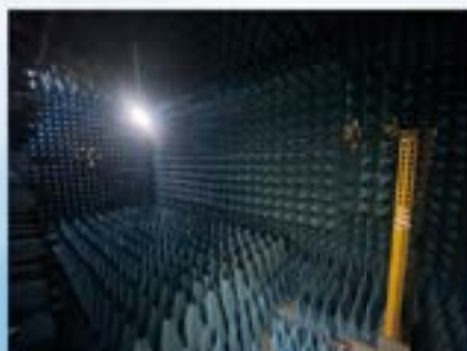
Antenna chamber for measuring gain value and efficiency of antennas
