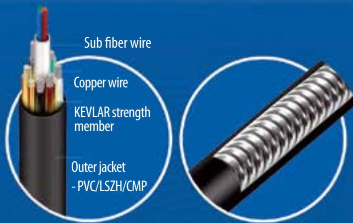
Ultra-thin armored AOC
