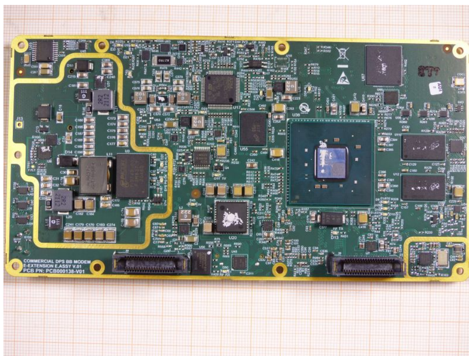
Photo 16: PCB000138
