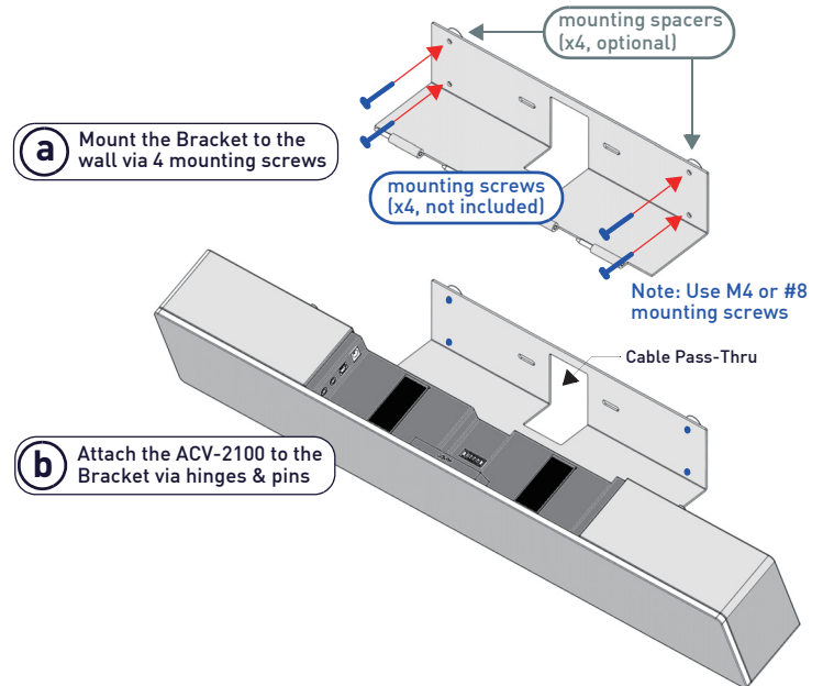
FIG. 4 WALL MOUNTING THE ACV-2100
