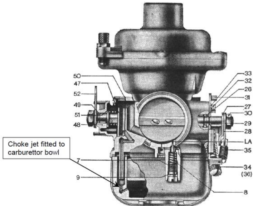
Figure 50 – Choke Schematic
