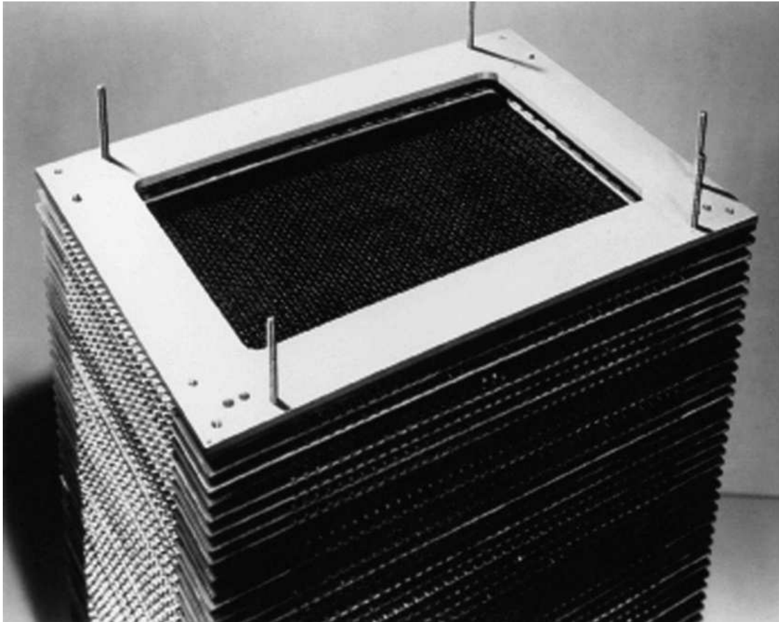
FIGURE E5.17.2 A core memory plane from the Whirlwind containing 256 cores arranged in a 16 \times 16 array.
