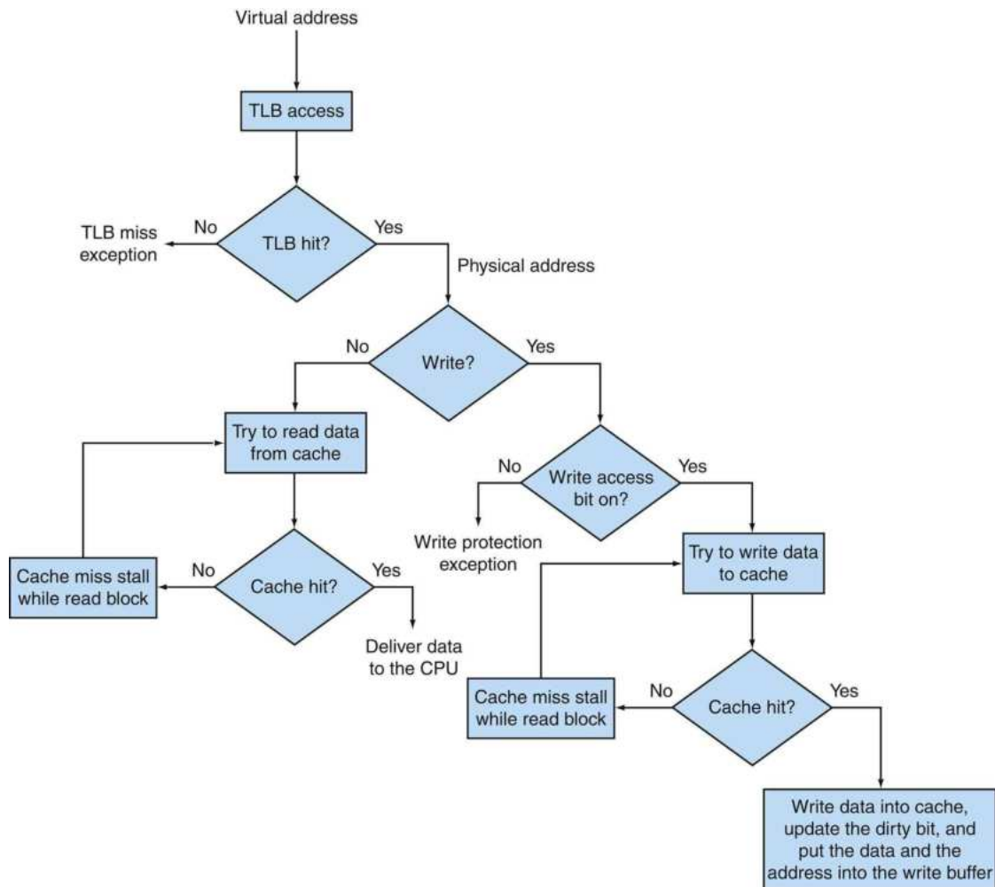
FIGURE 5.32 Processing a read or a write-through in the Intrinsic FastMATH TLB and cache.
