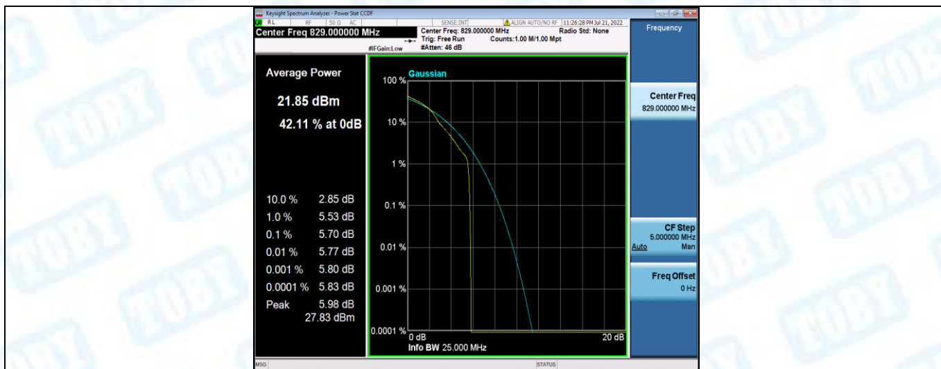
Band5-10MHz-16QAM-20450-50RB#0
