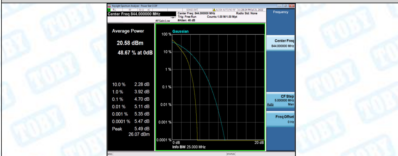
Band5-10MHz-16QAM-20450-1RB#0
