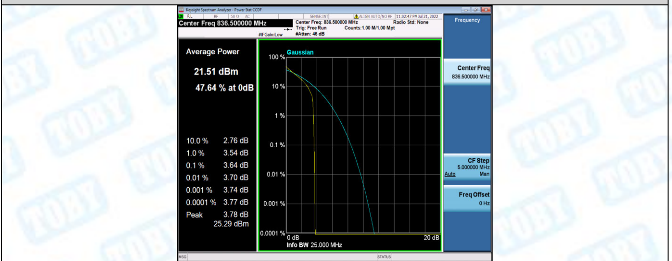
Band5-5MHz-QPSK-20525-25RB#0
