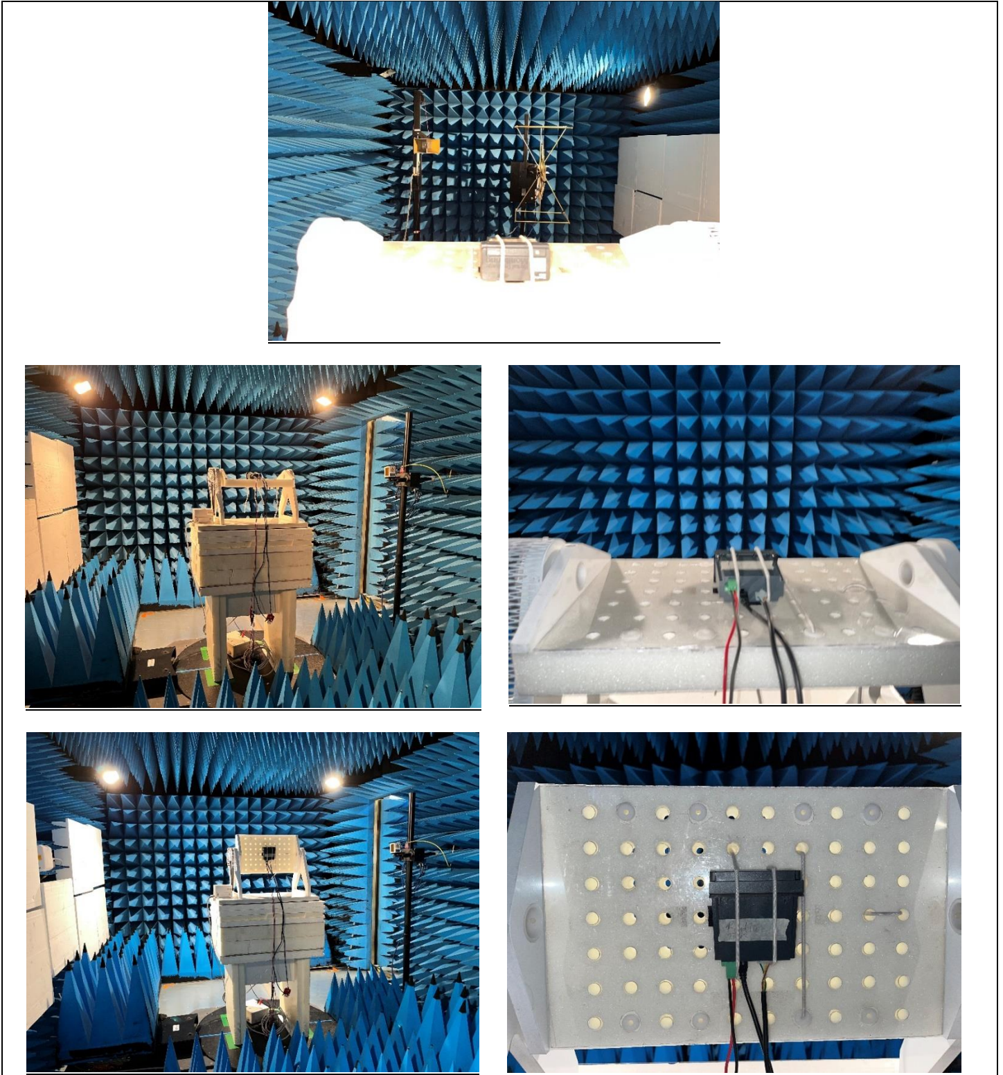
Photograph for Unwanted Emission in restricted frequency bands on FAR
