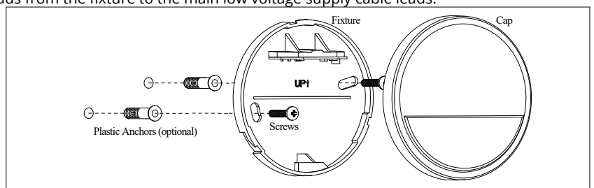
FIG. A Installation on Wall (most common use)
