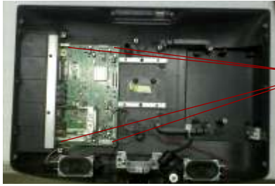
1.7The seventh of TV teardown --Tearing down the Main board
