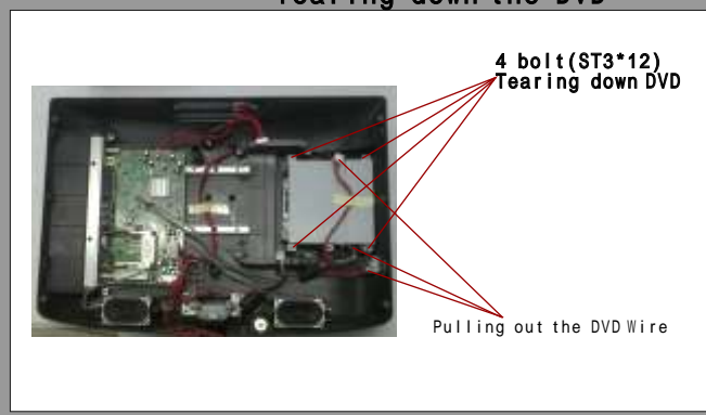
1.5The fifth of TV teardown --Tearing down the DVD
