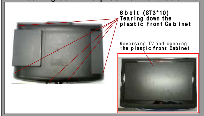
1.2.1The second of TV teardown --Tearing down the plastic front Cabinet
