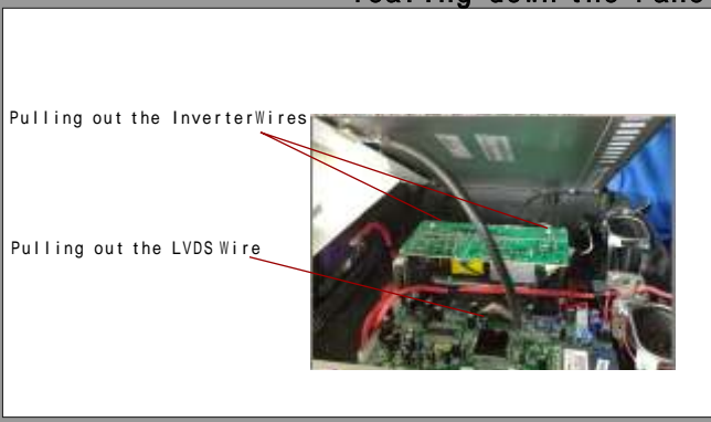
1.3.2The third of TV teardown --Tearing down the Panel
