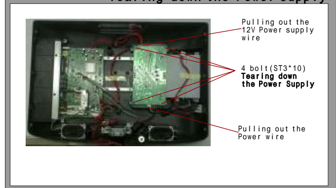
1.4The fourth of TV teardown --Tearing down the Power Supply
