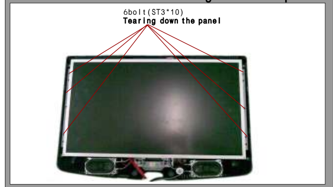
1.3.1The third of TV teardown --Tearing down the panel
