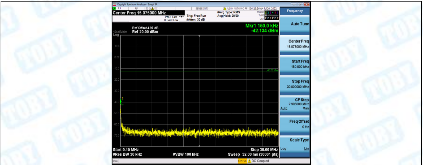
Band5-4183-4-1000~10000MHz
