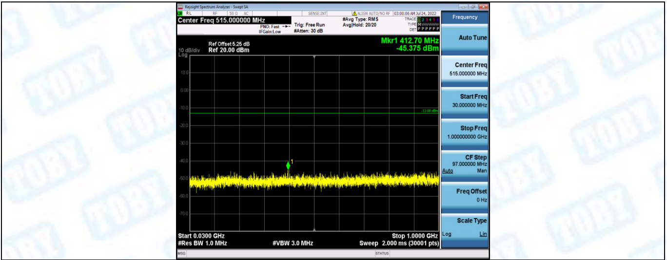
Band4-1413-4-0.009~0.15MHz
