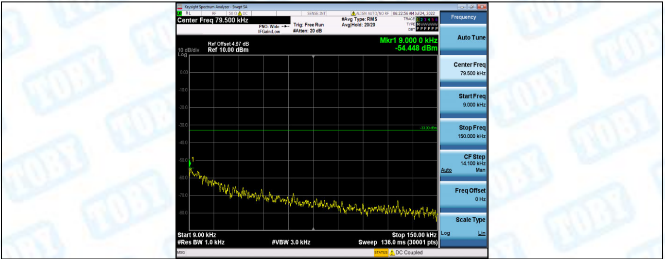
Band5-4183-4-0.009~0.15MHz
