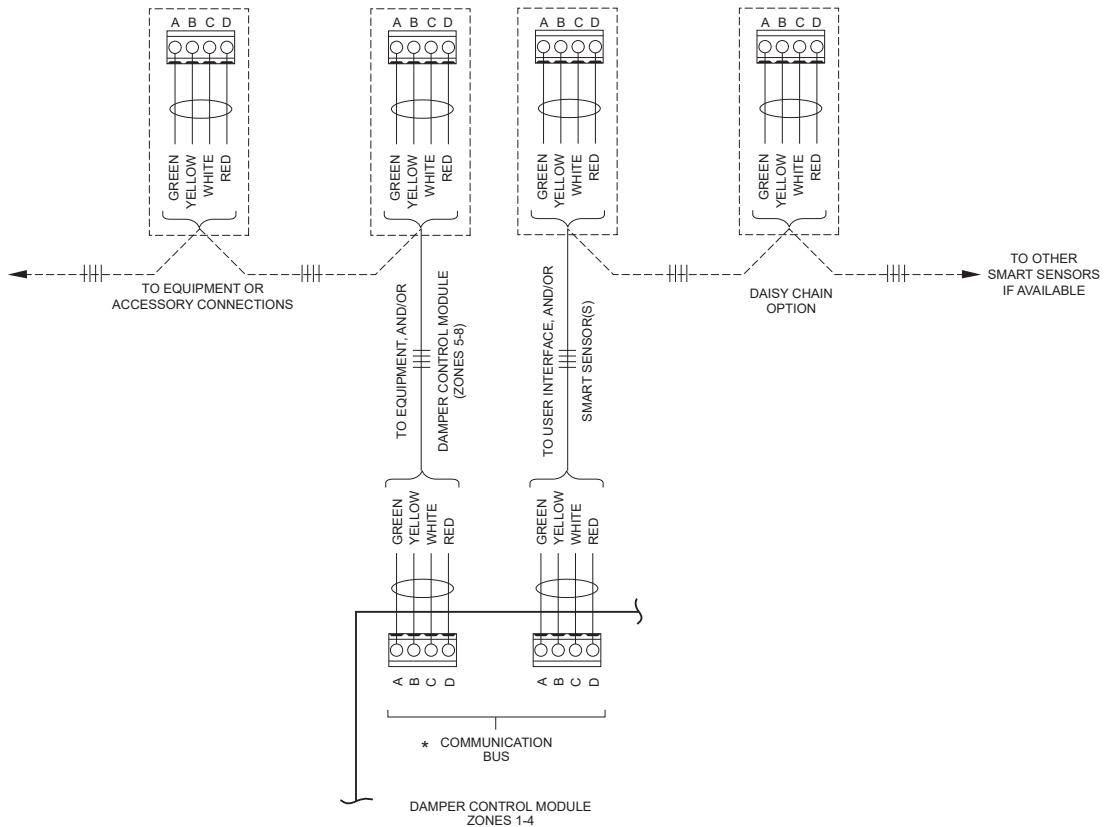
Fig. 2 – Typical Smart Sensor Wiring Diagram
