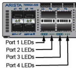
Figure A-2: Port LEDs
