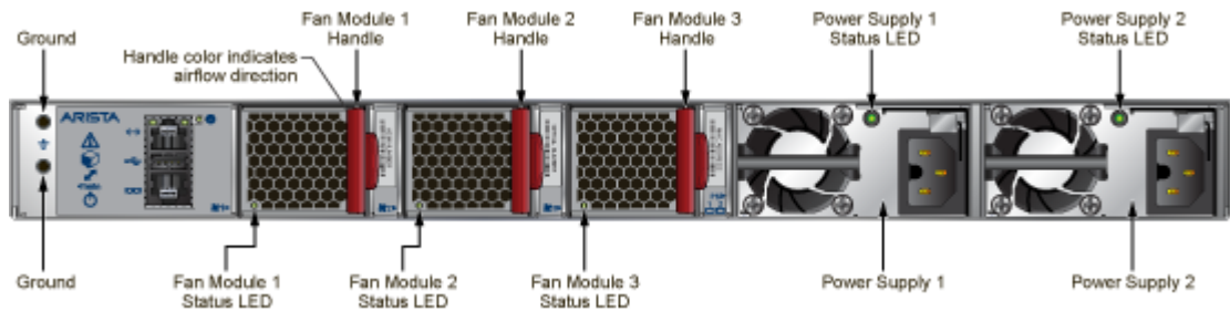
Figure D-1: Rear Panel for CCS-720XP-48ZC2
