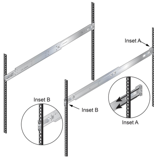
Figure 3-10: Attaching the Rails
