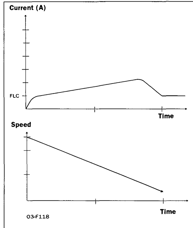
Fig. 36 Pump control
