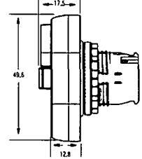
Non-Illuminated 3-Position Multi-Function Operators (D7x-U3)
