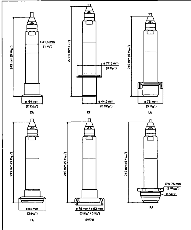
Fig. 18: VEGABAR 75 - hygienic fitting: CA/CF = Tri-Clamp 2"/Tri-Clamp 2½", LA = hygienic fitting with compression nut F40, TA = Tuchenhagen Varivent DN 32, R/RW = bolting DN 40/DN 50 according to DIN 11851, KA = conus DN 40, AA = DRD
