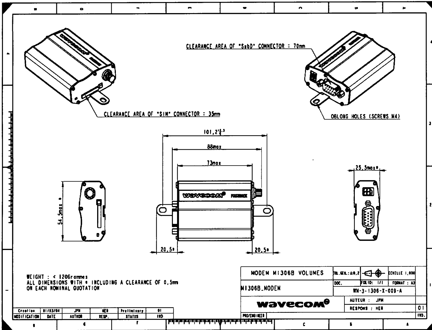
Figure 18: Dimensioning diagram
