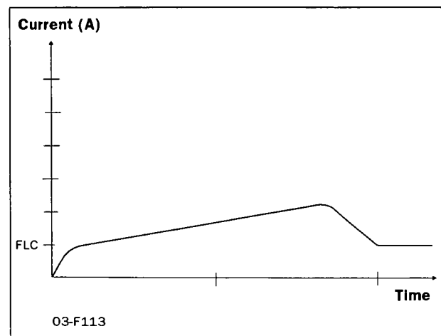
Fig. 5 Torque control
