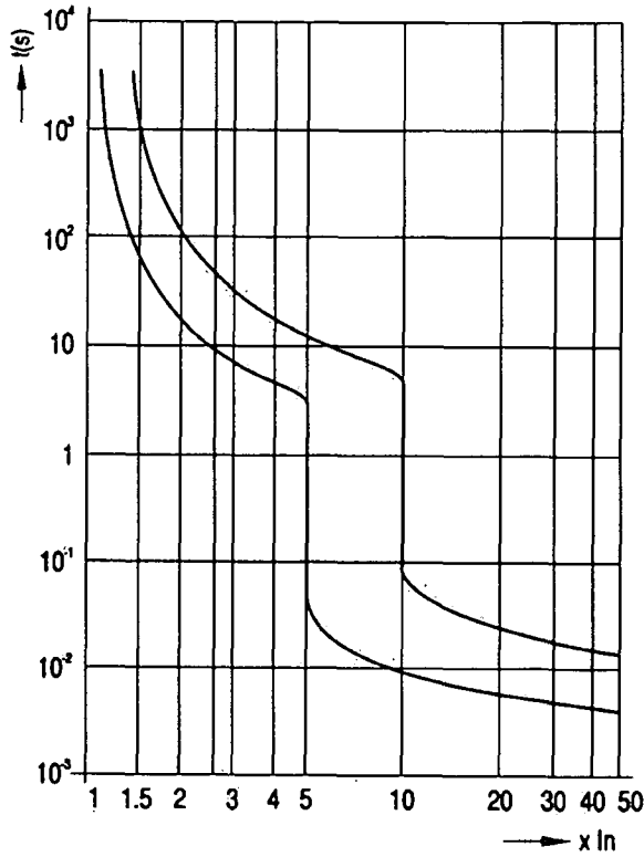
Curve C
