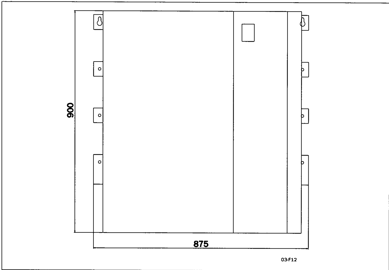
Fig. 22 MSF -1000 to -1400
