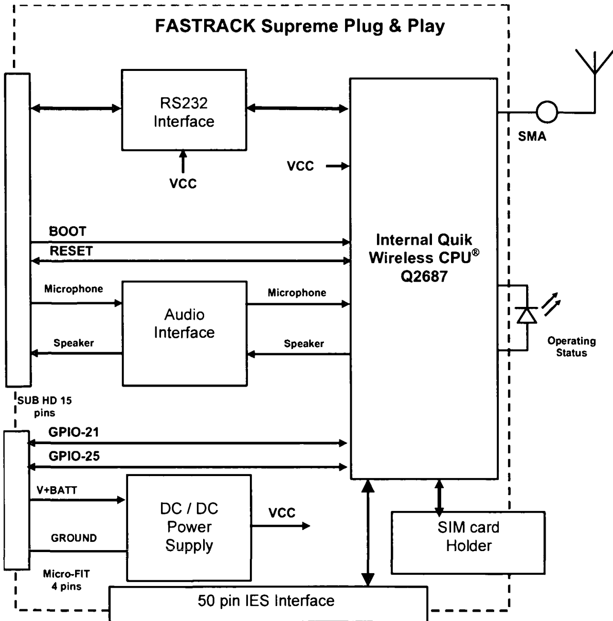
Figure 15: Functional architecture
