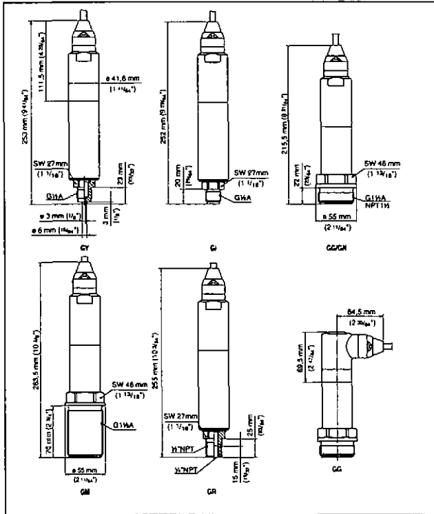
Fig. 11: VEGABAR 74 - threaded fitting: GV = G \frac{1}{2} A manometer connection EN 837, GI = G \frac{1}{4} A inner G \frac{1}{4} A, GG = G \frac{1}{2} A, GN = 1 \frac{1}{2} NPT, GM = G \frac{1}{2} A 70 mm
