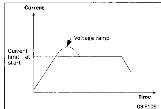
Fig. 34 Current limit
