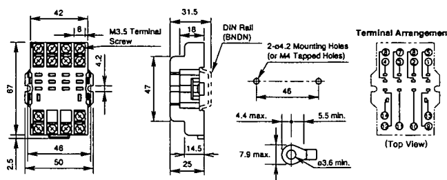
SH4B-05
