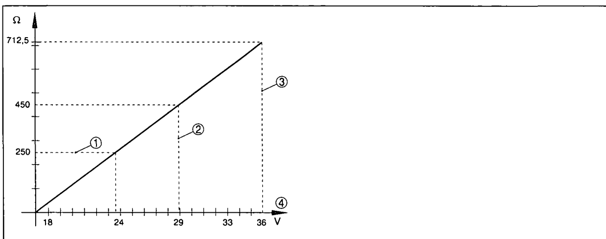
Fig. 10: Voltage diagram
