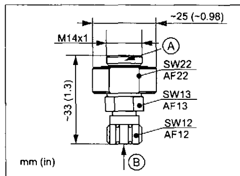
Testing adapter
