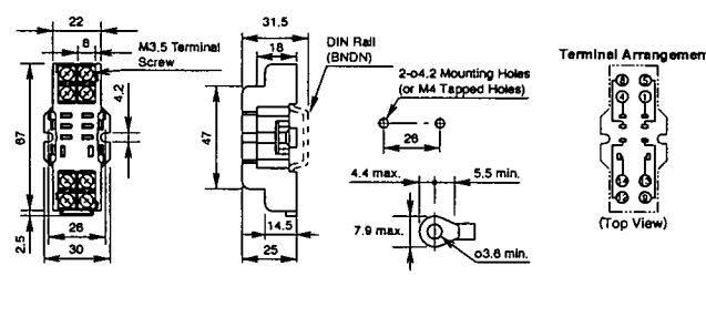
SH4B-05
