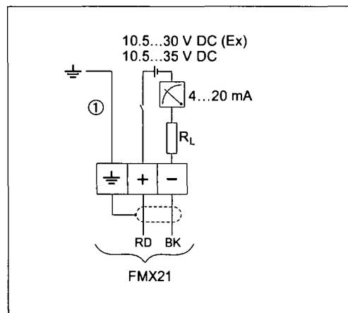
Electrical connection
