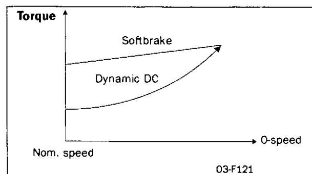
Fig. 46 Braking time
