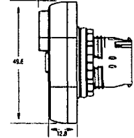
Toggle Switch Operators (D7M-JM)
