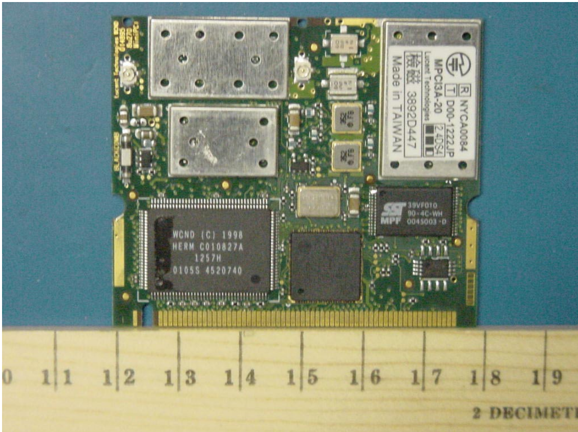
PHOTOGRAPH 13-5: TOP VIEW
