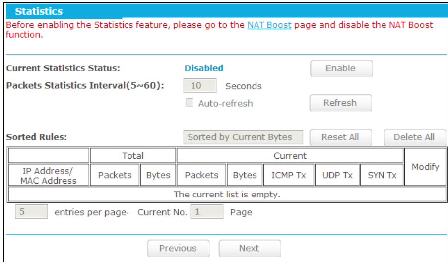
Figure 5-118 Statistics
