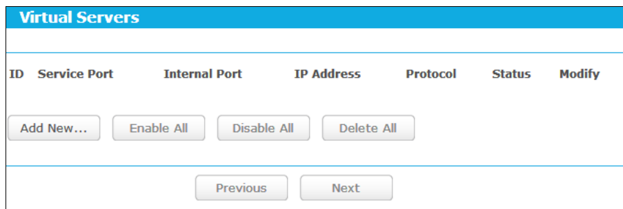
Figure 5-51 Virtual Servers
