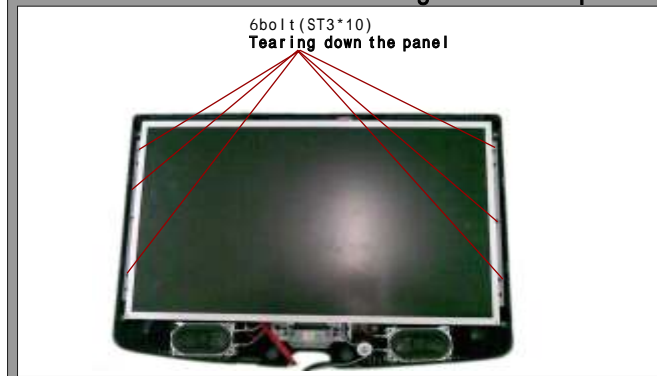
1.3.1The third of TV teardown --Tearing down the panel
