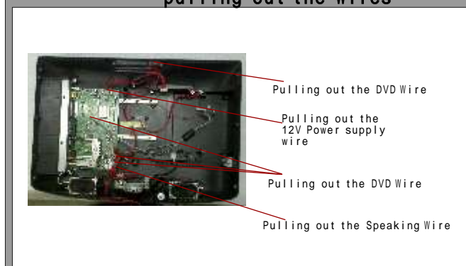
1.6The sixth of TV teardown --pulling out the Wires
