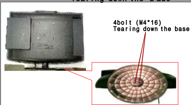
1.1The first of TV teardown --Tearing down the base
