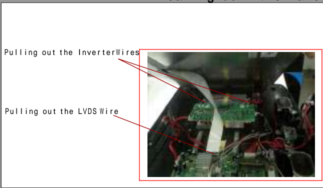
1.3.2The third of TV teardown --Tearing down the Panel
