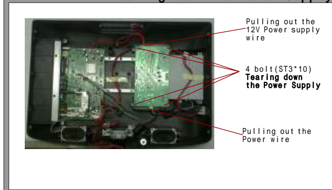
1.4The fourth of TV teardown --Tearing down the Power Supply
