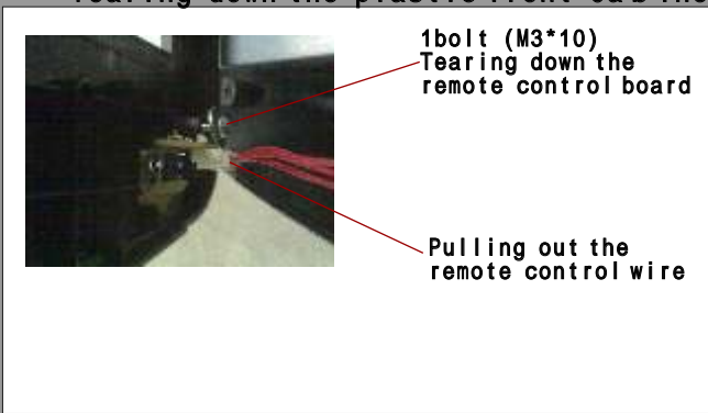
1.2.2The second of TV teardown --Tearing down the plastic front Cabinet
