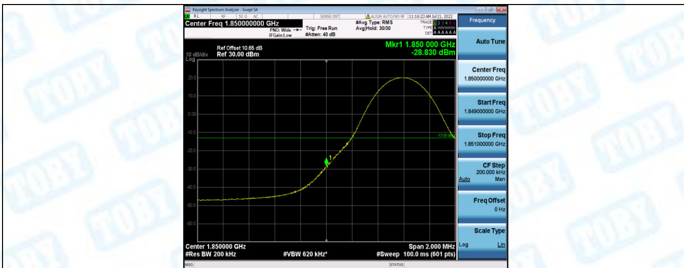
Band2-10MHz-16QAM-18650-1RB#49
