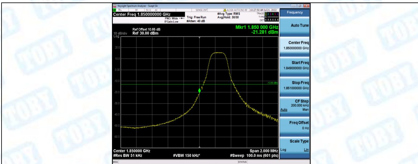
Band2-3MHz-16QAM-18615-1RB#14
