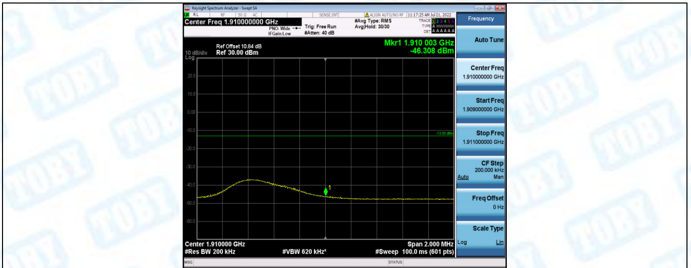
Band2-10MHz-QPSK-19150-1RB#49
