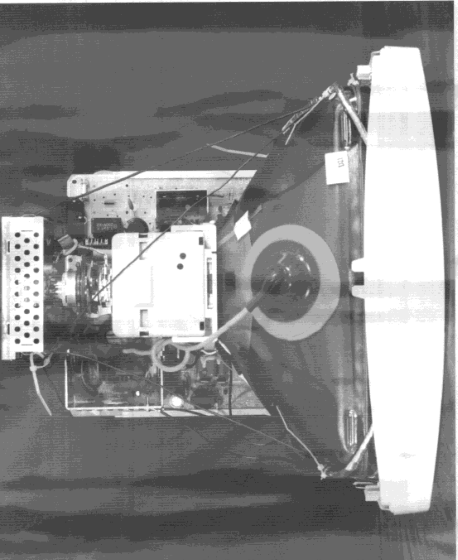
Top View w/o Back Cover
