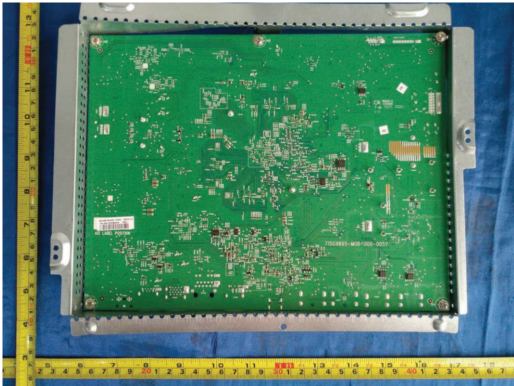
Figure 10. Internal view of metal enclosure for main board
