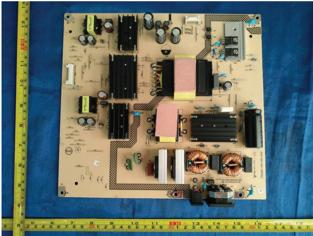
Figure 11. Power board 715GA067
