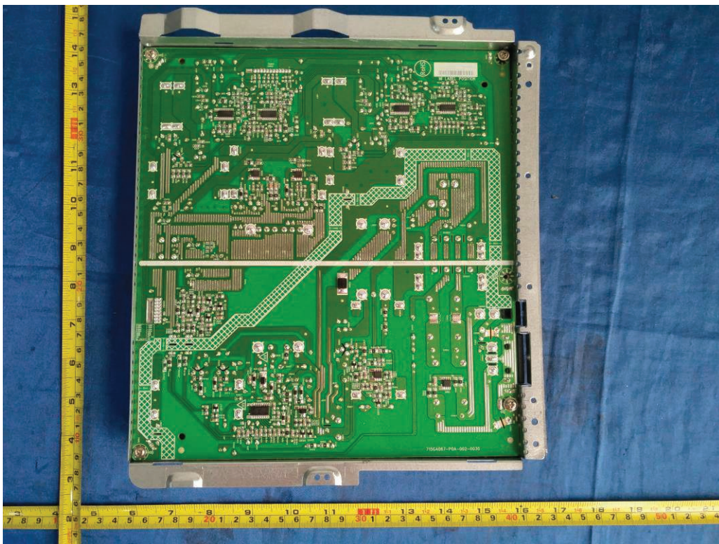
Figure 8. Internal view of metal enclosure for power board
