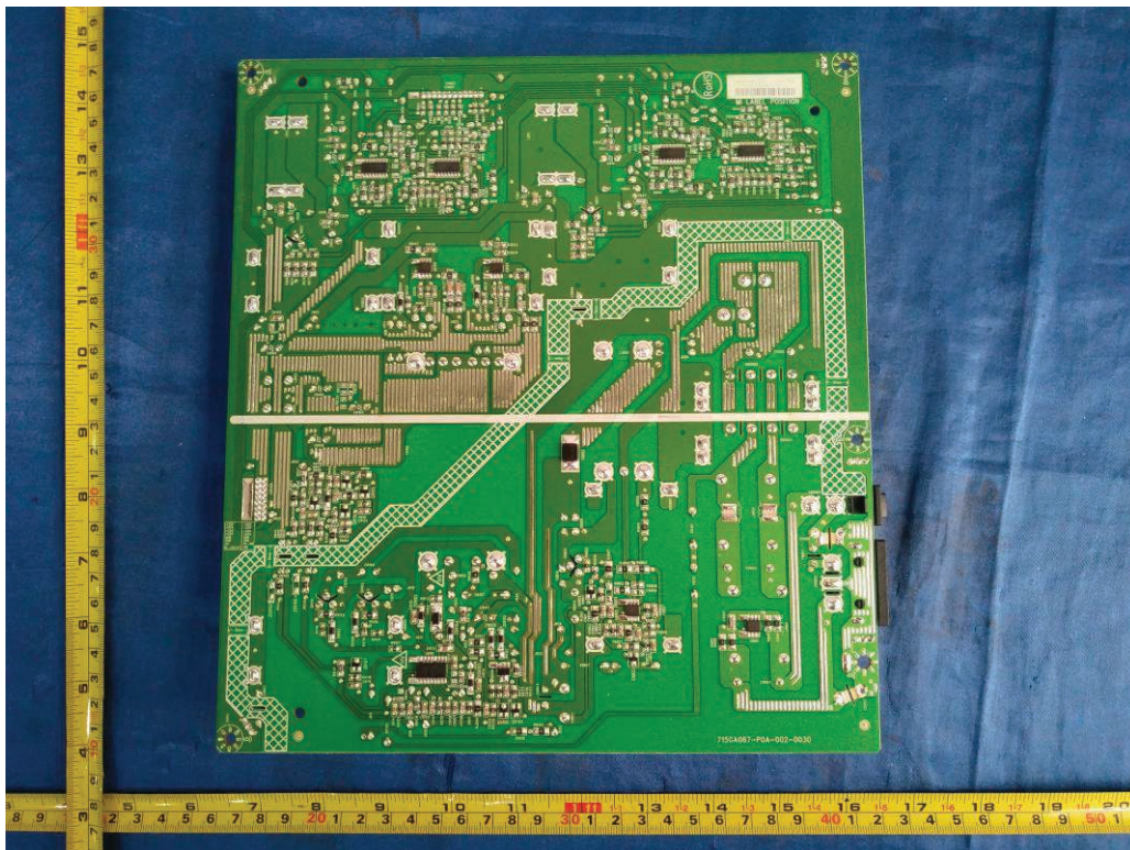
Figure 12. Power board 715GA067
