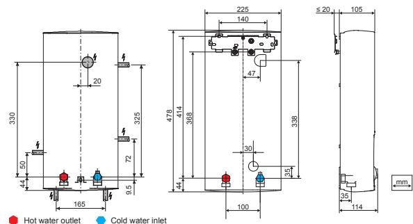
DHB-E 13 AU 50°C instantaneous 3 phase electric water heater
