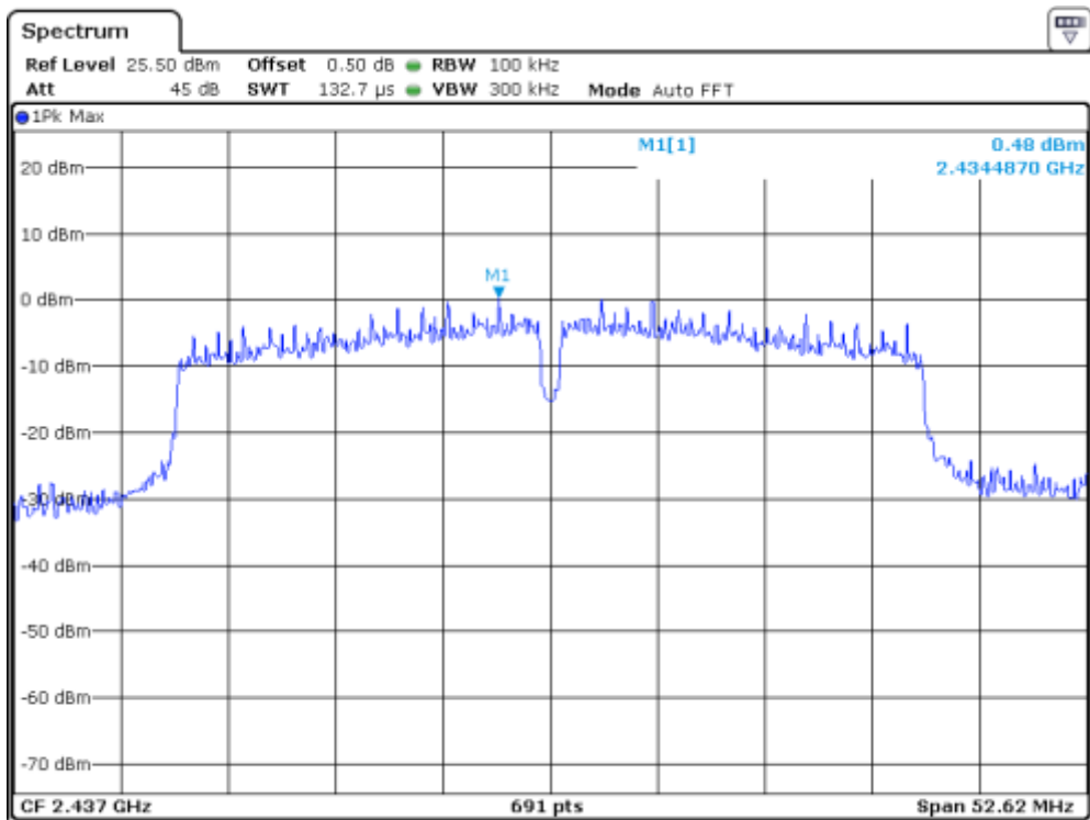
Channel 06 (2437MHz) Reference Level: 0.48dBm
