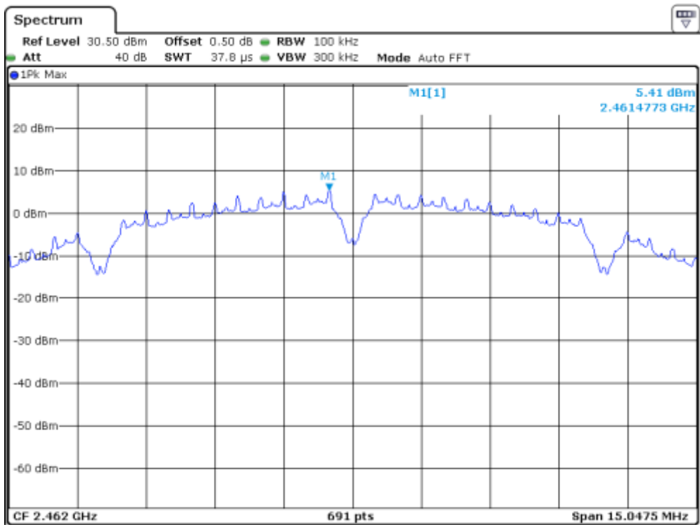
Channel 11 (2462MHz) Reference Level: 5.41dBm
