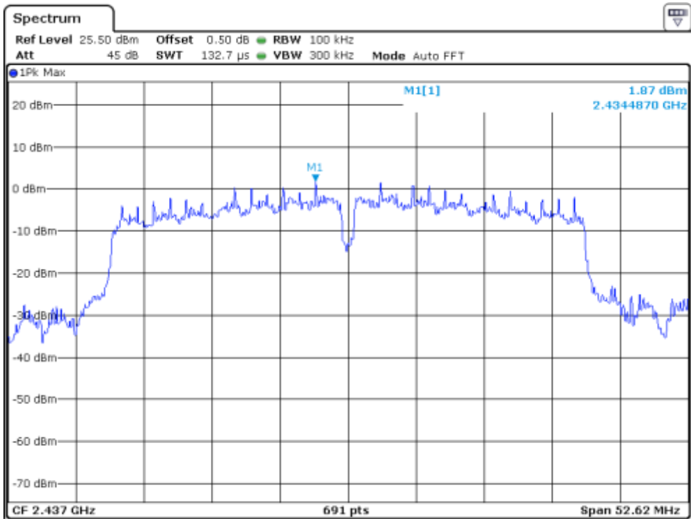
Channel 06 (2437MHz) Reference Level: 1.87dBm
