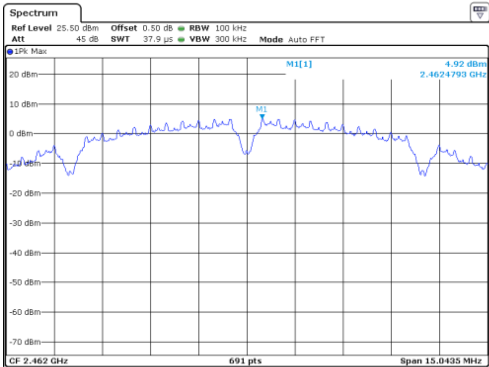
Channel 11 (2462MHz) Reference Level: 4.92dBm
