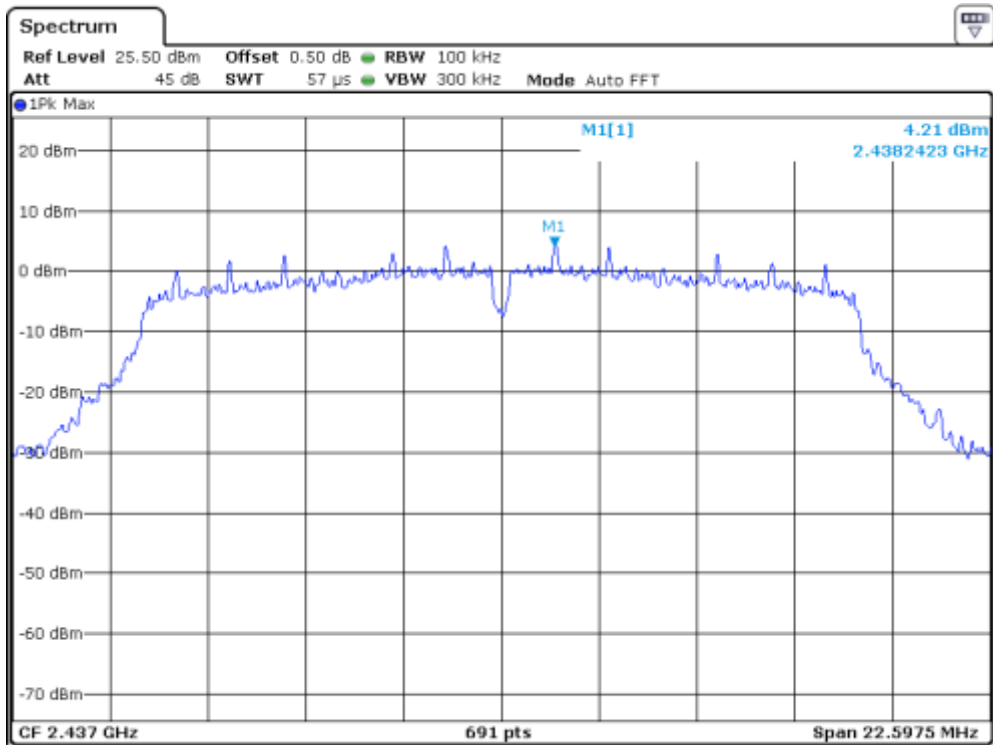
Channel 06 (2437MHz) Reference Level: 4.21dBm
