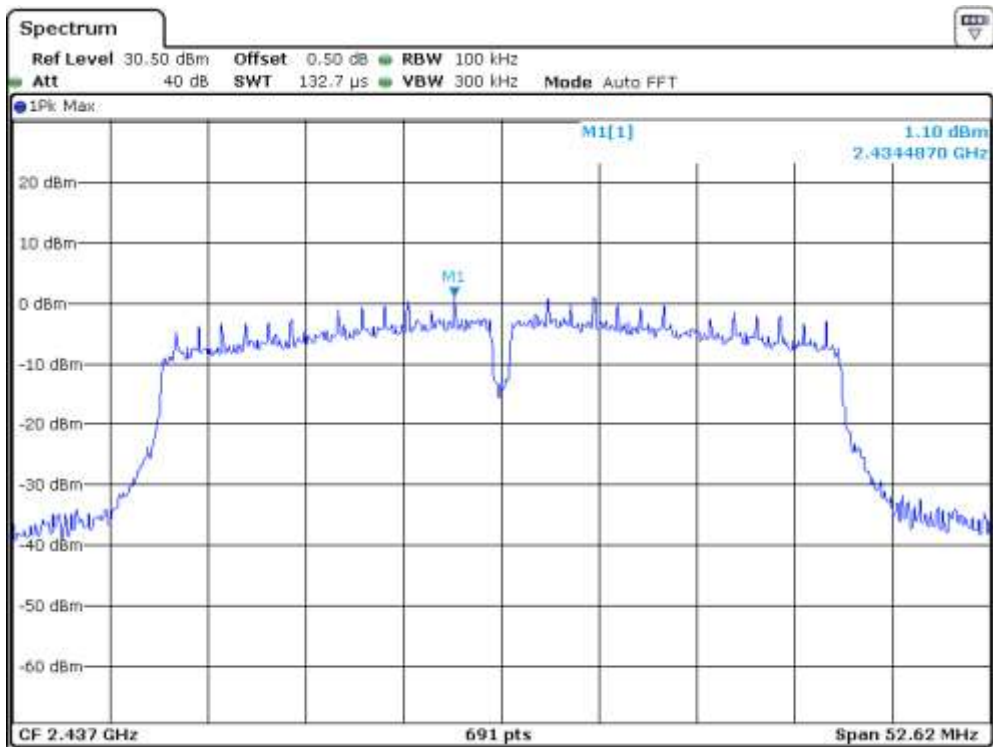
Channel 06 (2437MHz) Reference Level: 1.10dBm
