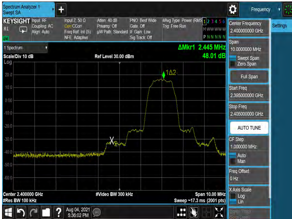
Plot 7-25. Band Edge Plot Antenna WF7 (Bluetooth with Hopping Disabled, 8DPSK, ePA – Ch. 0)
