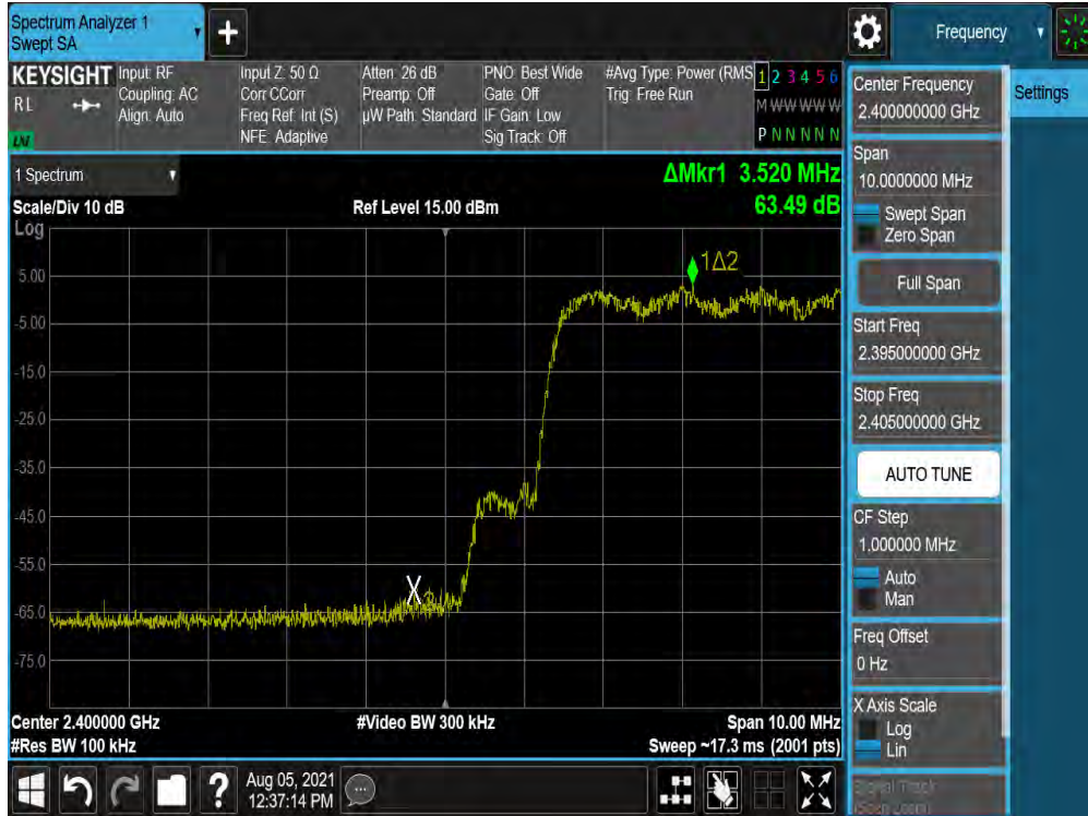
Plot 7-27. Band Edge Plot Antenna WF7 (Bluetooth with Hopping Enabled, 8DPSK, ePA)
