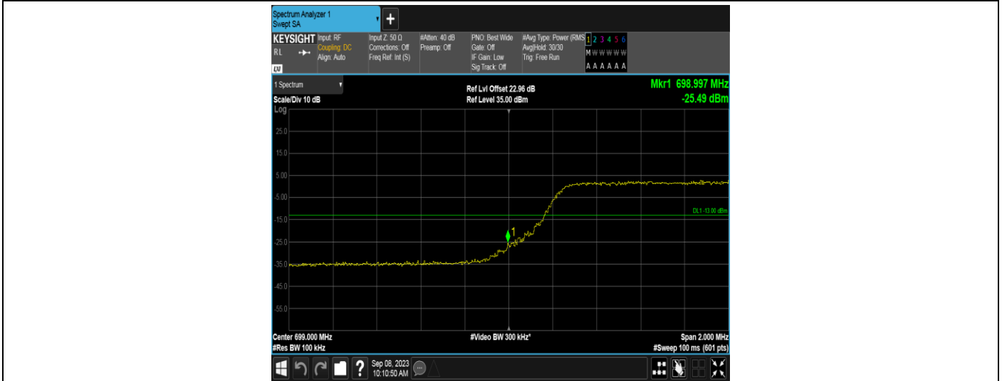
Band12-5MHz-16QAM-23155-1RB#0
