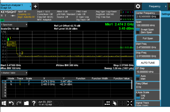
Hopping enabled_ High Channel 2473MHz-2573MHz
