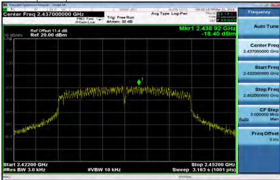
802.11n_HT20 PSD (CH-Mid)
