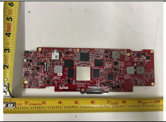
Main board Front View
