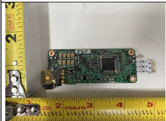
PCB2 Rear View
