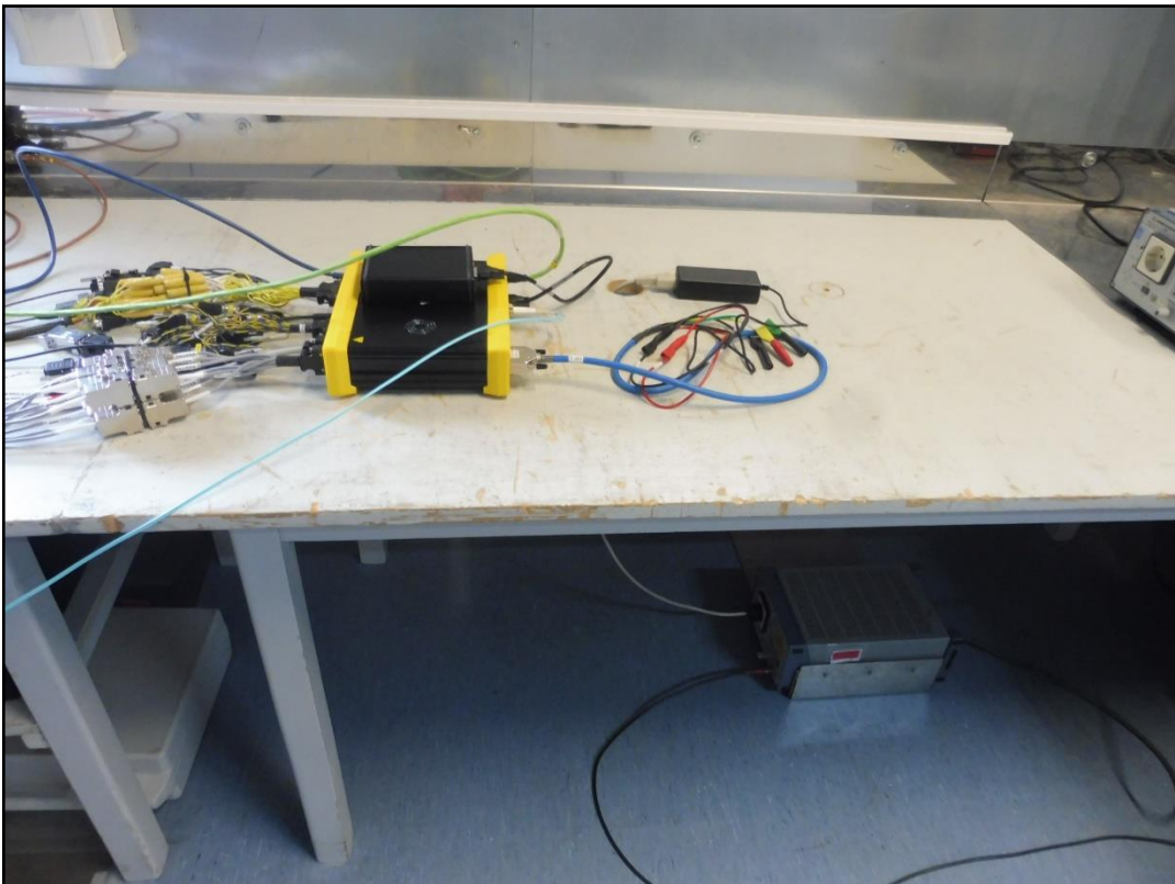
Photo 10: conducted emission
