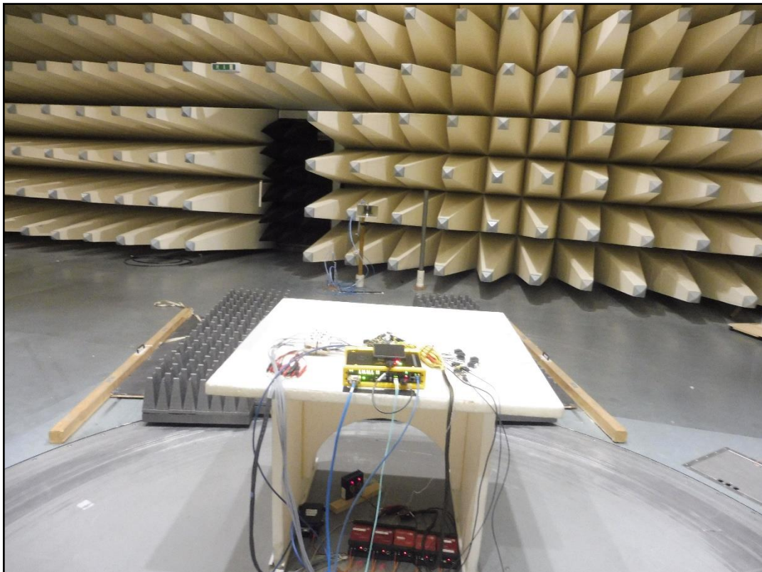
Photo 4: radiated emission
