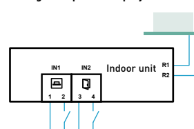
Wiring example for display controller.
