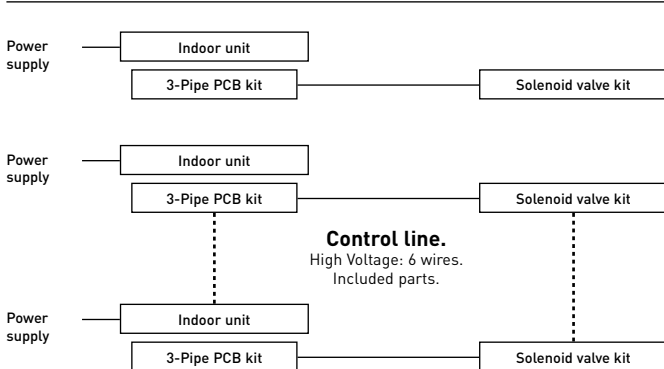
3-Pipe PCB kit. Separately purchased.
