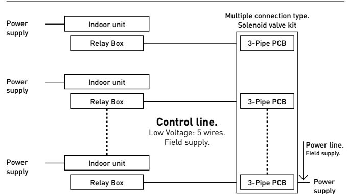
Signal Relay Box. Included accessory.
