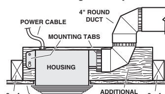
HOUSING MOUNTED TO 2x4 TRUSS Requires additional framing for mounting tabs. Discharge 90° to joists.
