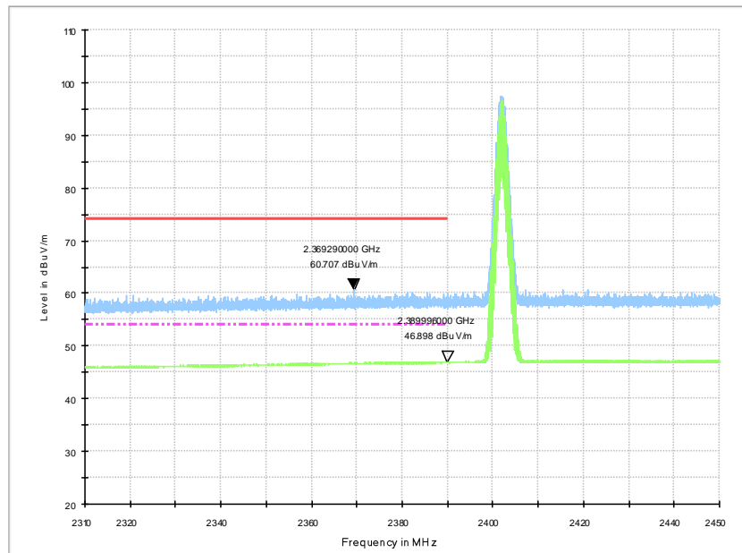
Fig.13. Frequency Band Edges: GFSK, Channel 0, 2.31 GHz – 2.45GHz
