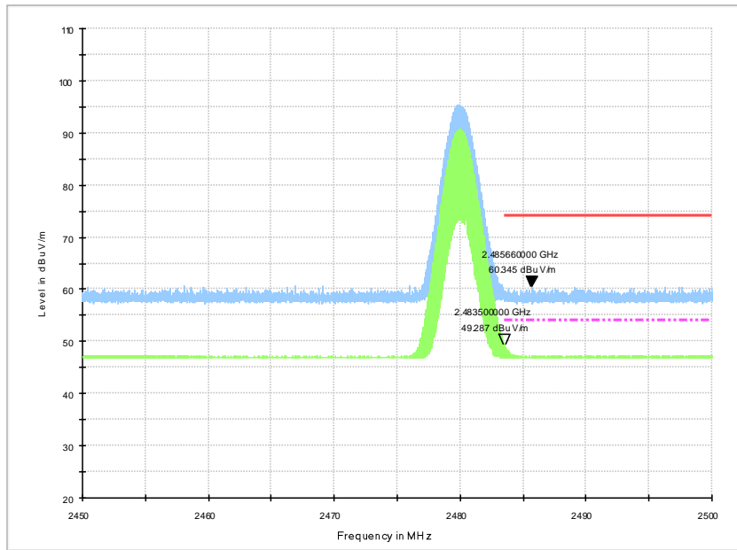
Fig.18. Frequency Band Edges: 8DPSK, Channel 78, 2.45 GHz - 2.50GHz
