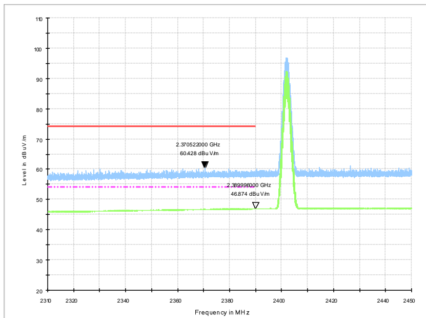
Fig.15. Frequency Band Edges: \pi/4 DQPSK, Channel 0, 2.31 GHz - 2.45GHz
