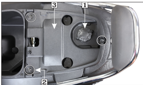
(1) Fuel filler cap (2) Bolts (3) Fuel tank cover
