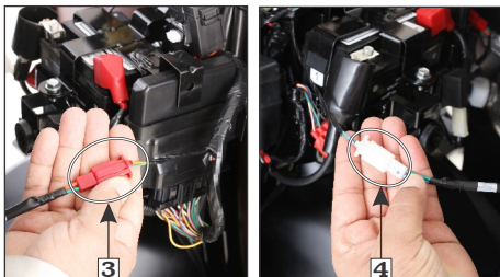
(3) Left turn signal lamp connector (4) Right turn signal lamp connector
