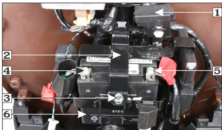
(1) Fuse box (2) Battery clamp (3) Bolt (4) (-)ve terminal (5) (+)ve terminal (6) Battery
