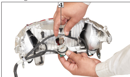
(4) Tail/stop lamp bulb
