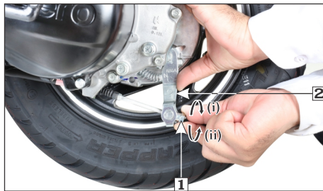
(1) Adjuster nut (2) Brake arm (i) Decrease free play (ii) Increase free play
