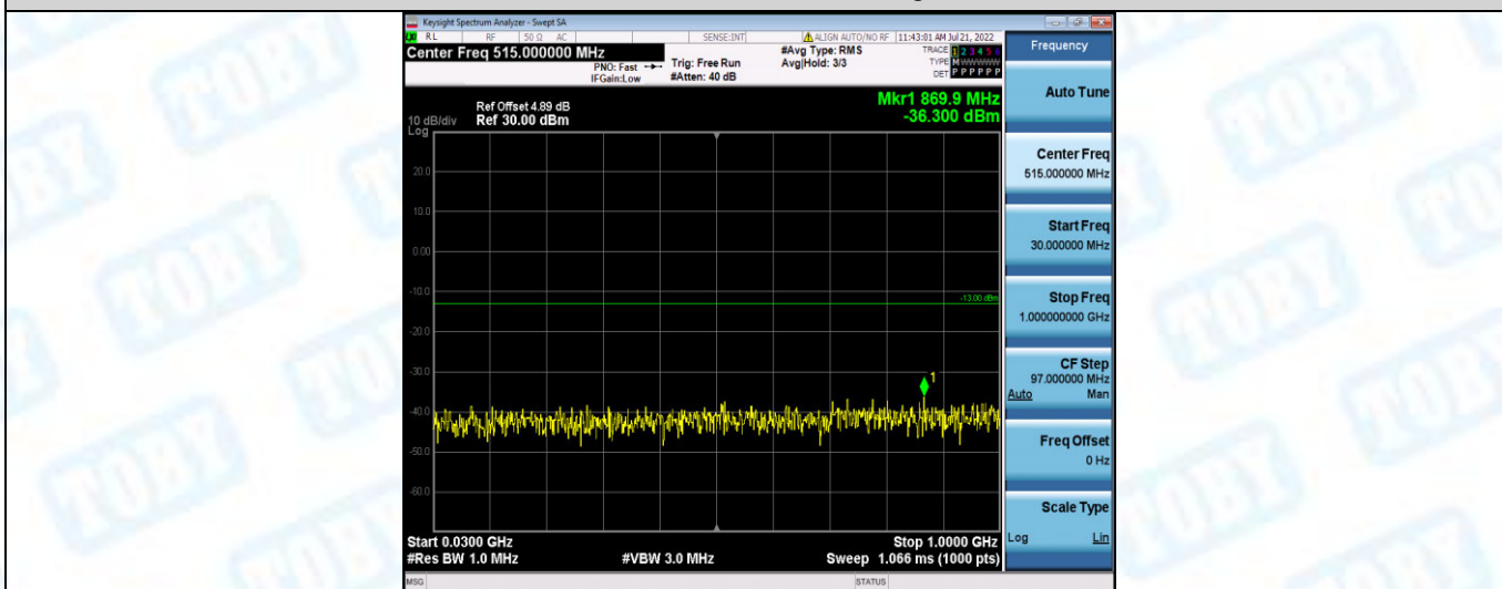
Band2-15MHz-QPSK-18900-1RB#0-Range2:1000~2000MHz
