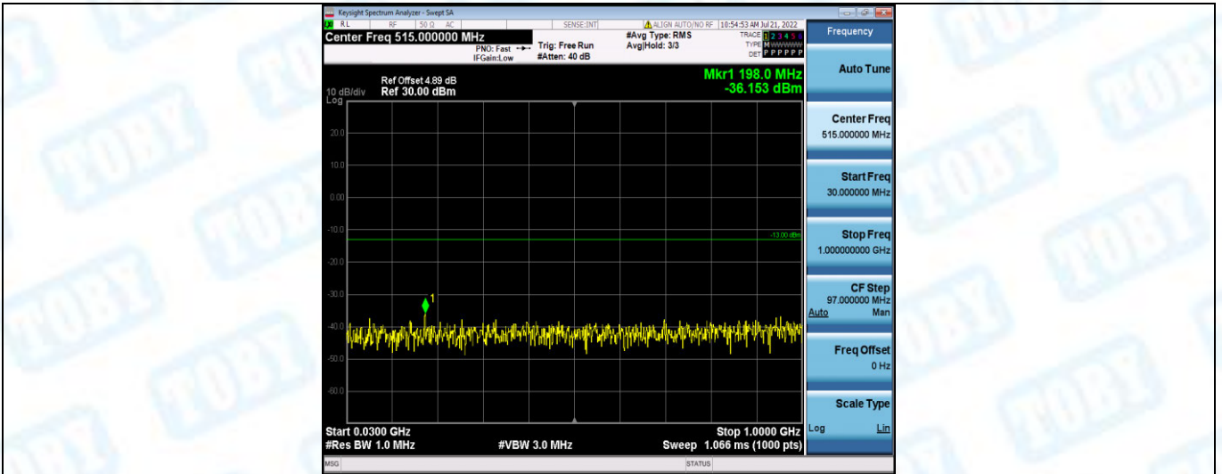
Band2-5MHz-16QAM-18625-1RB#0-Range2:1000~2000MHz
