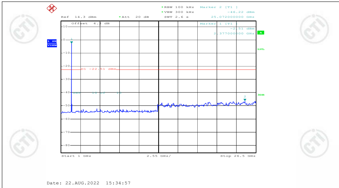
BLE_1M_Ant1_2402_1000~26500
