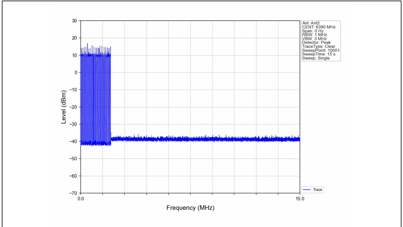
802.11ax(HEW40)_HCH_6405MHz_Inject signal_6420MHz_ - Inject Incumbent signal at 10th seconds and keep the signal continuously injected
