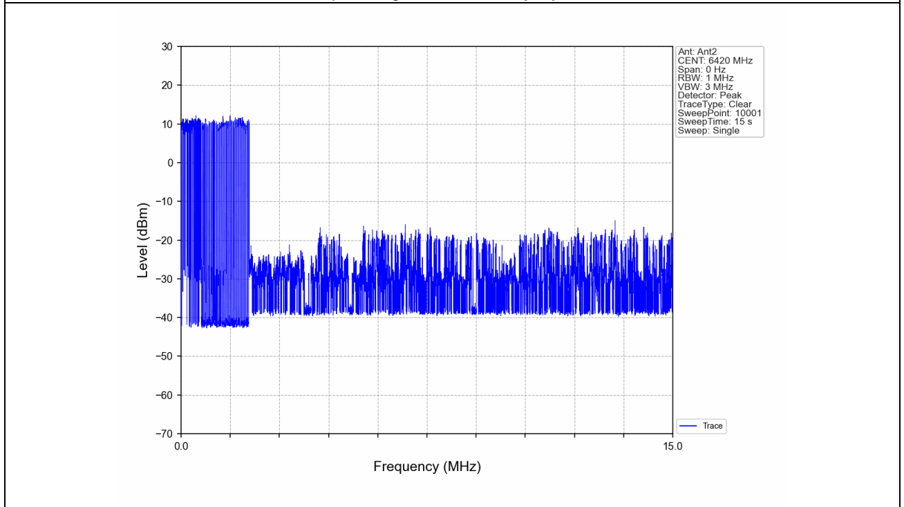
802.11ax(HEW80)_HCH_6385MHz_Inject signal_6420MHz_ - Inject Incumbent signal at 10th seconds and
