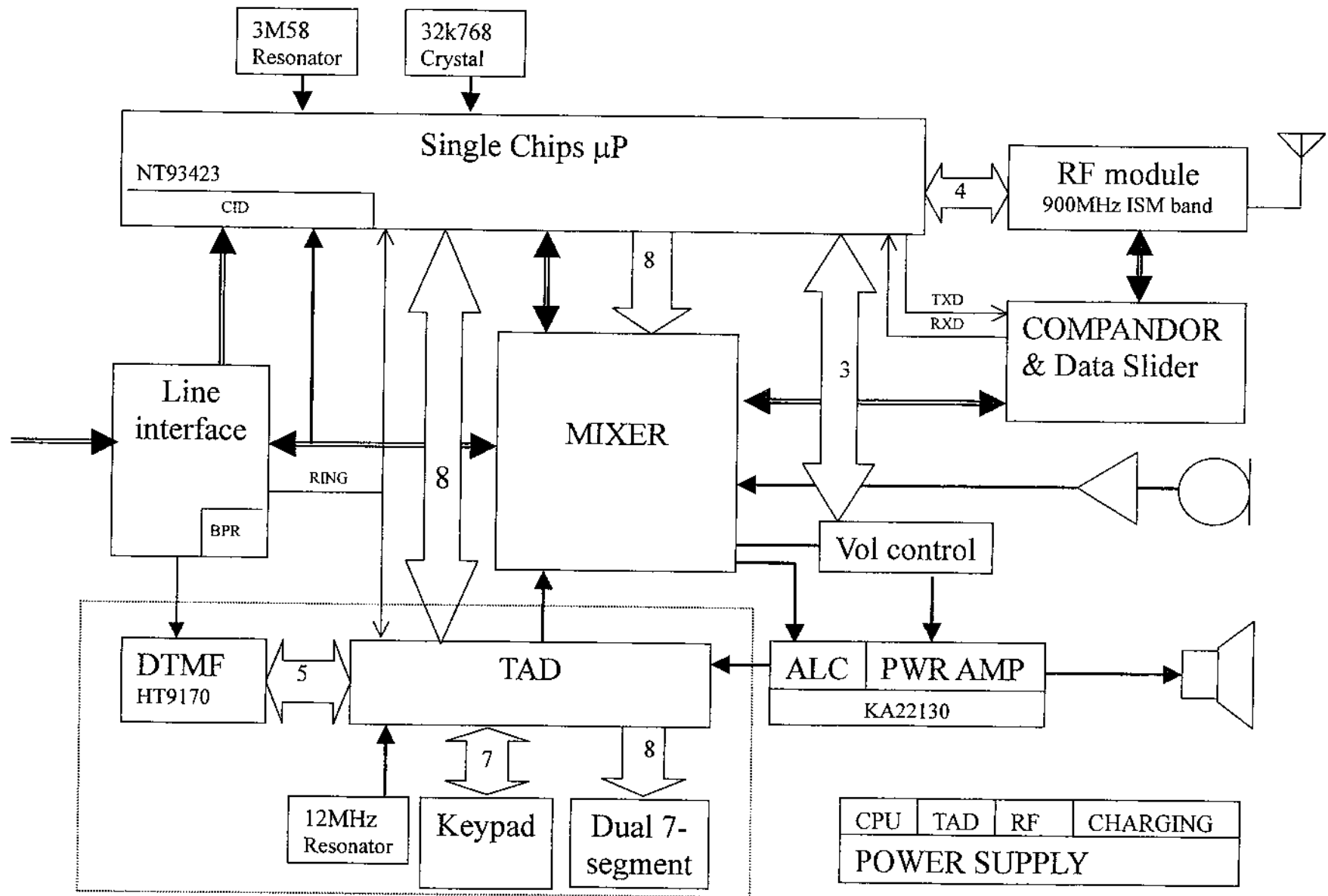
FF2150 900MHz phone Base block diagram
