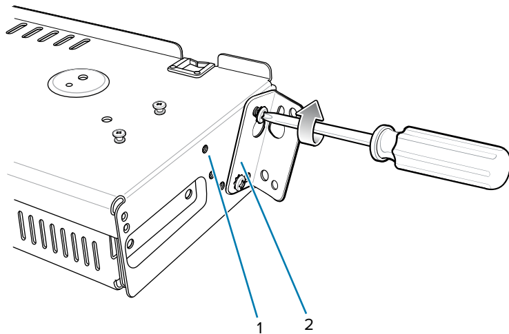
Figure 52 Flange 25° Position (4-Slot Battery Chargers)
