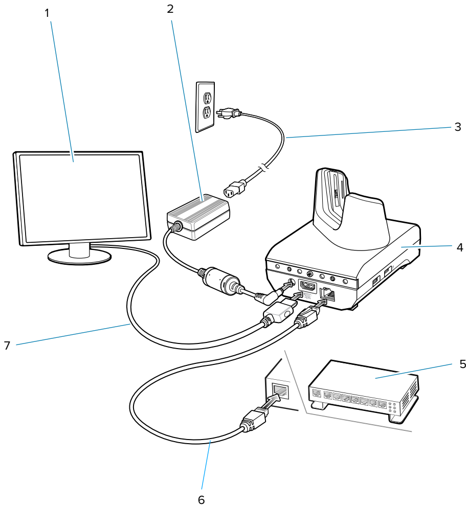
Figure 37 Workstation Cradle Setup
