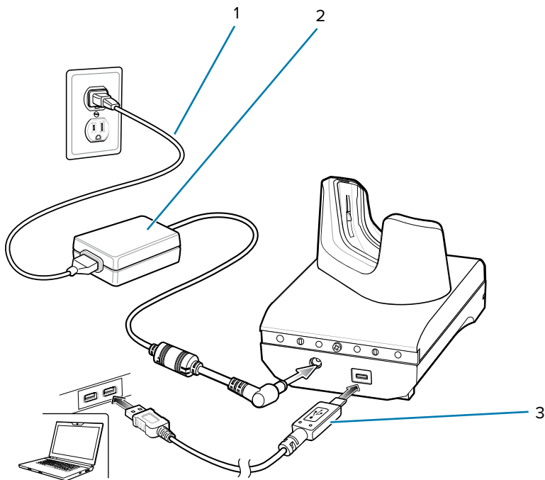
Figure 35 1-Slot USB Charge Cradle Setup
