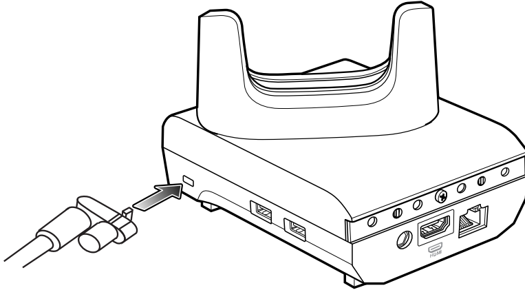
Figure 38 Securing Cradle with Kensington Lock
