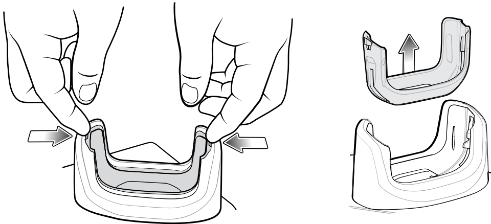
Figure 48 Remove the Insert from the Cup
