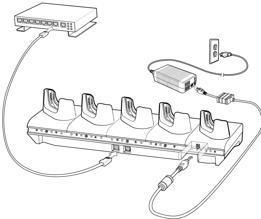
Figure 47 5-Slot Ethernet Cradle Setup
