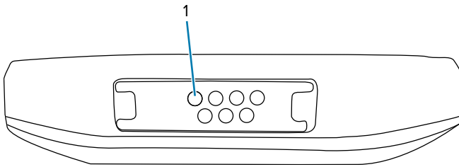
Figure 53 I/O Connector Pin-Outs
