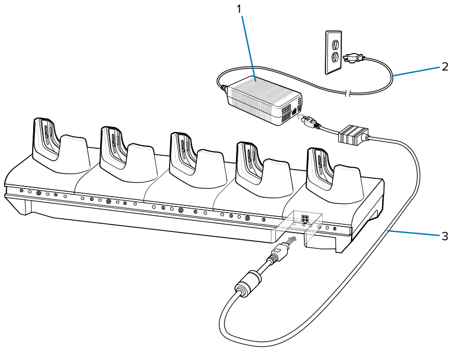
Figure 44 5-Slot Charge Only Cradle Setup
