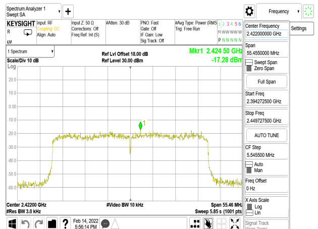
802.11ax_40MHz_Chain1_2422MHz
